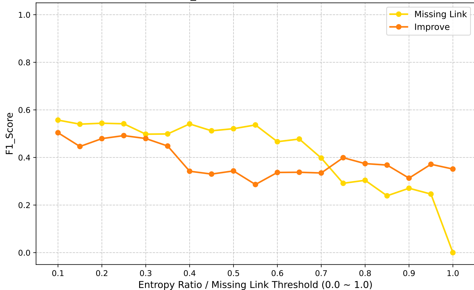
F1_Score (Global Round: 20)
