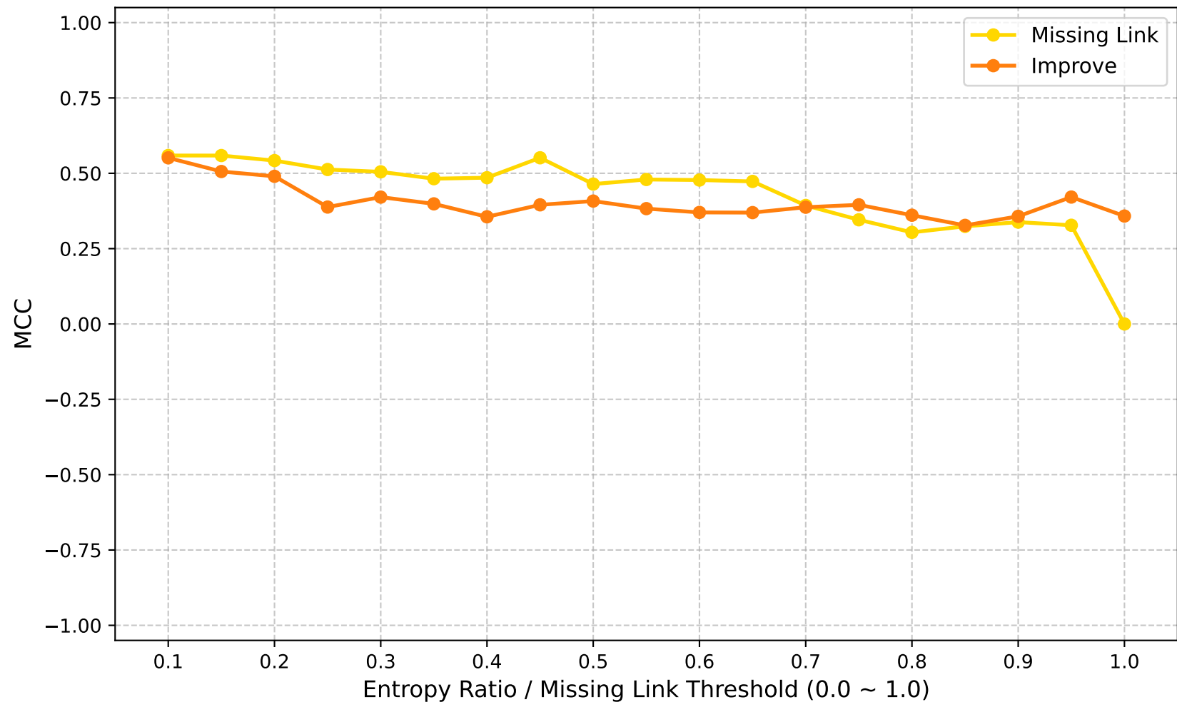
MCC (Global Round: 5)
