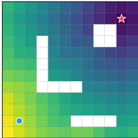
(b) Goal distance field
