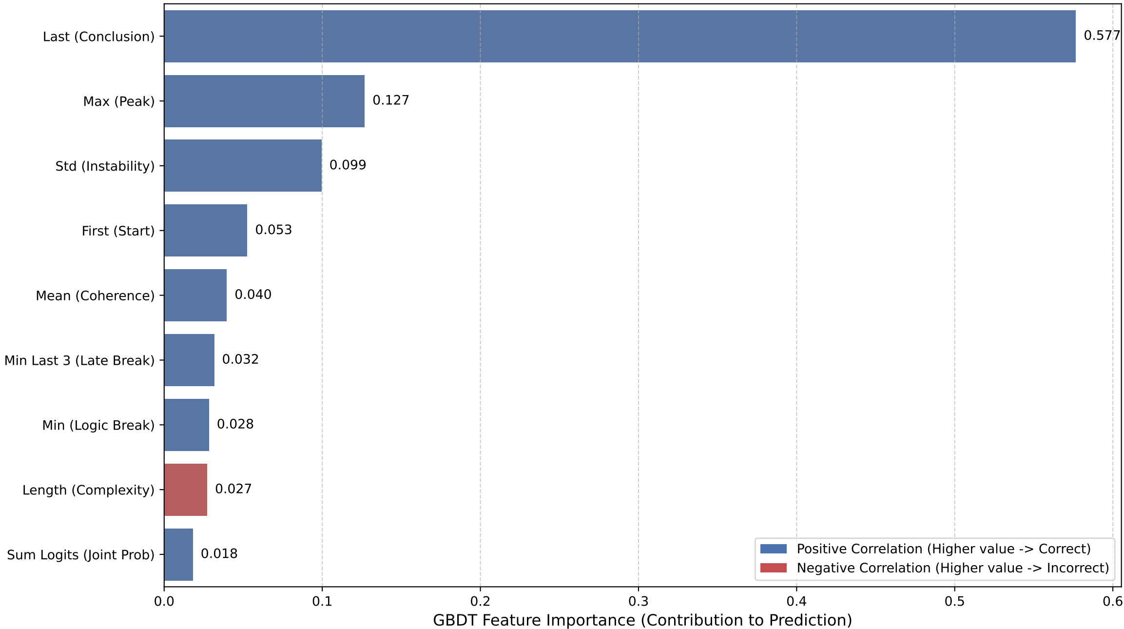
Features extracted from Step Scores
