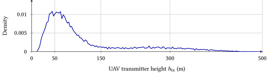
Figure 3.1: Empirical UAV transmitter height density read directly from the CKM HDF5 database using the 3 m histogram of Eq. (3.1), linearly interpolated between bin centres for display. Most training support lies in the low and mid-altitude bands.
