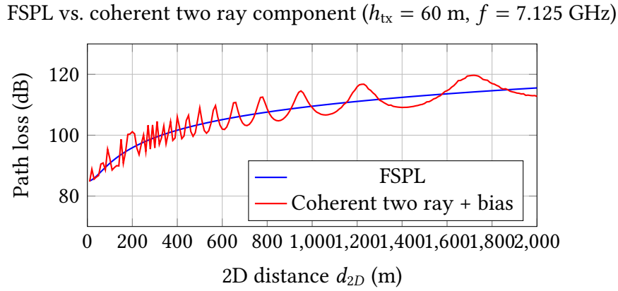
Figure 3.6: Schematic comparison of FSPL and the calibrated coherent two ray component for a 60 m UAV at 7.125 GHz ( h_{rx} = 1.5 m). The plotted red curve uses the code-loaded 60 m calibration values before adding the radial residual profile, so it shows the constructive/destructive interference term rather than the full final LoS prior.
