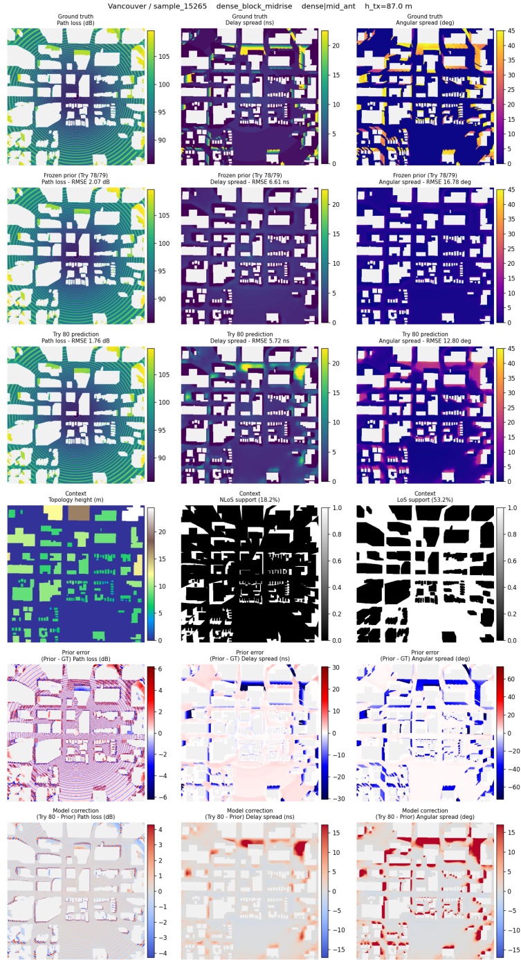
Figure 4.2: Representative final model inspection panel for a dense, mid altitude, held out test sample in Vancouver. This panel is kept here because it shows the final prior, residual correction and prediction side by side.
