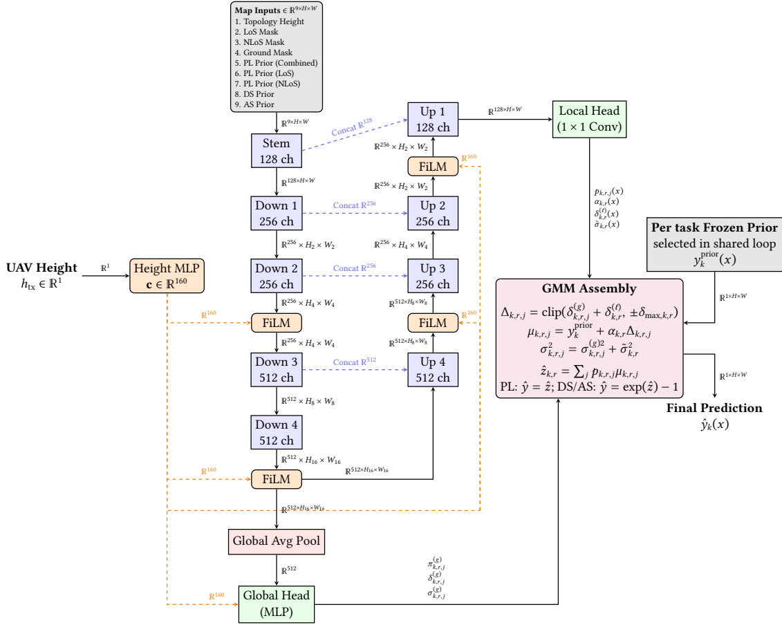
Figure D.7: Schematic of the final large capacity shared UNet architecture with FiLM conditioning. The backbone and decode logic are shared, while each task uses its own heads and frozen prior.
