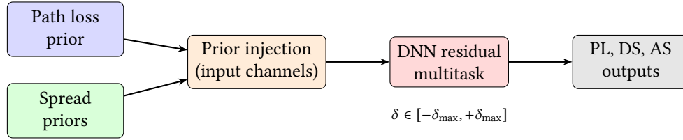
Figure 3.3: HARP-NET CKM pipeline. The frozen priors are injected into the DNN, which learns a bounded correction \delta around them.
