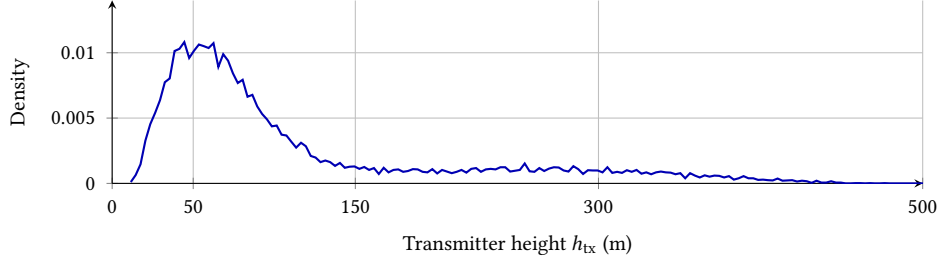
Figure 3.1: Empirical transmitter height density read directly from the CKM HDF5 database using the 3 m histogram of (3.1), linearly interpolated between bin centres for display. Most training support lies in the low and mid-altitude bands.
