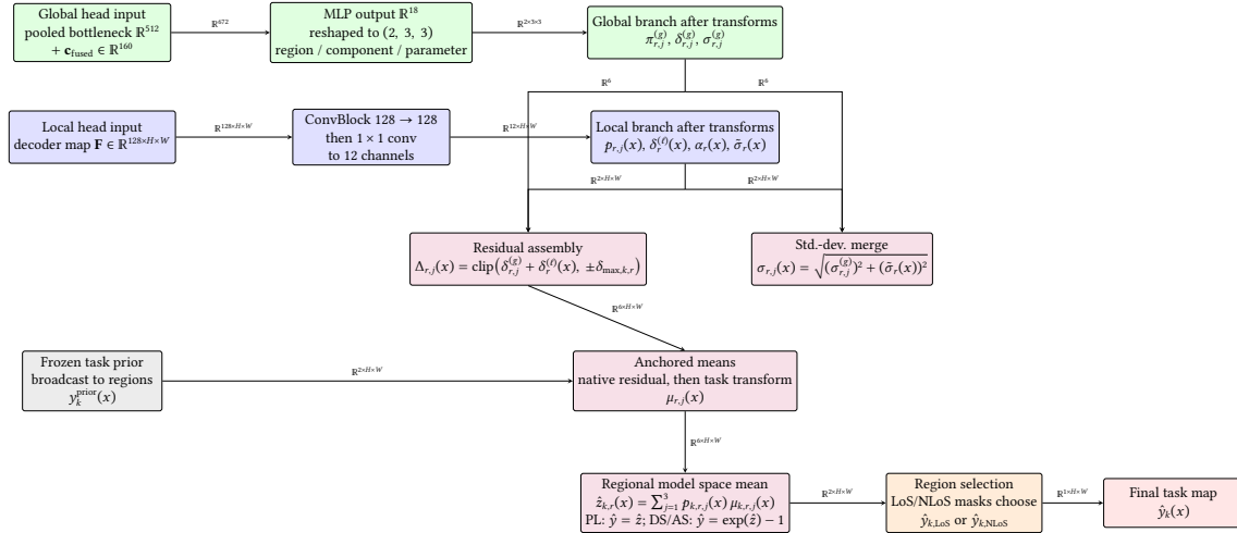
Figure D.9: Detailed HARP-NET CKM residual head used by the final model.
