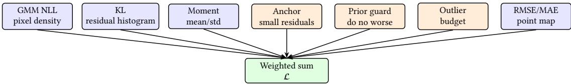
Figure D.10: Composite final loss family. In the final residual fine tuning stage, the selected final model keeps the GMM head and uses RMSE/MAE, anchor and guard penalties; NLL, KL, moment and outlier budget weights are set to zero. Earlier residual stages used nonzero probabilistic weights.
