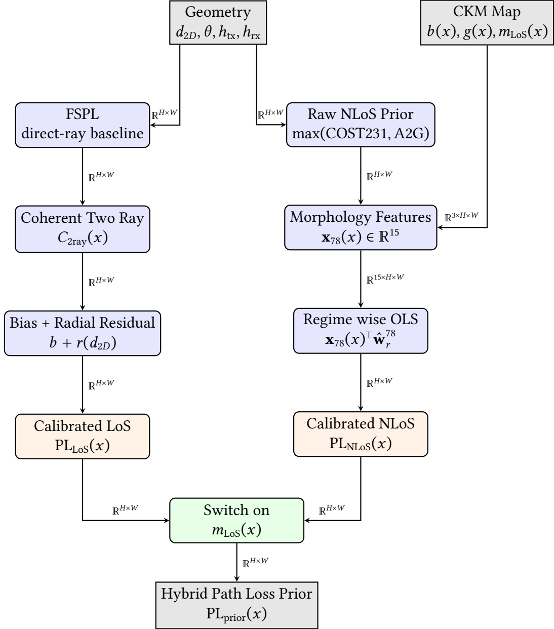
Figure D.4: Pipeline for the hybrid path loss prior. The LoS branch relies on an explicit two ray interference model, while the NLoS branch calibrates a raw prior against map derived morphology features using regime wise OLS. The two branches are hard-switched based on the LoS mask to produce the final frozen prior.
