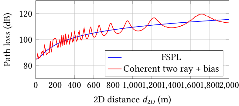
Figure D.3: Schematic comparison of FSPL and the calibrated coherent two ray component for a 60 m UAV at 7.125 GHz ( h_{\text{rx}} = 1.5 \text{ m} ). The plotted red curve uses the code-loaded 60 m calibration values before adding the radial residual profile, so it shows the constructive/destructive interference term rather than the full final LoS prior.
