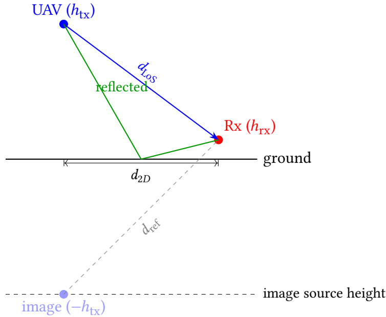
Figure 3.5: Two ray geometry. Direct path (blue) has length d_{\text{LoS}} ; reflected path (green) has the same total length as the image source path (gray dashed), which is d_{\text{ref}} .
