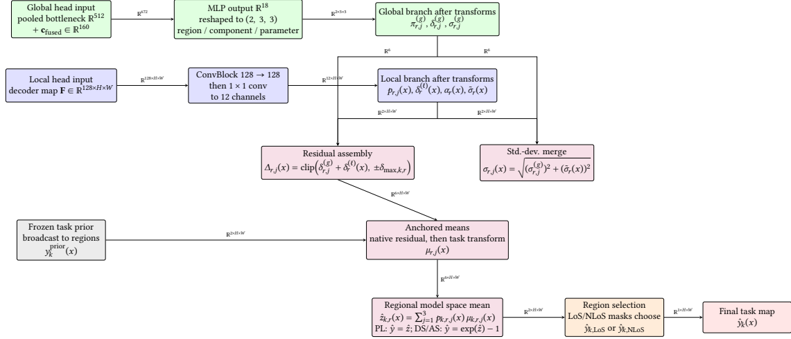
Figure 3.12: Detailed HARP-Net CKM residual head used by the final model.
