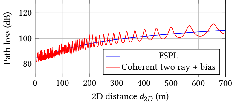
Figure 3.7: Schematic comparison of FSPL and the calibrated coherent two ray component for a 60 m UAV at 7.125 GHz ( h_{\text{rx}} = 1.5 \text{ m} ), zoomed to the 700 m near field that contains the full 513 \times 513 map diagonal. The plotted red curve uses the code loaded 60 m calibration values before adding the radial residual profile, so it shows the constructive/destructive interference term rather than the full final LoS prior.
