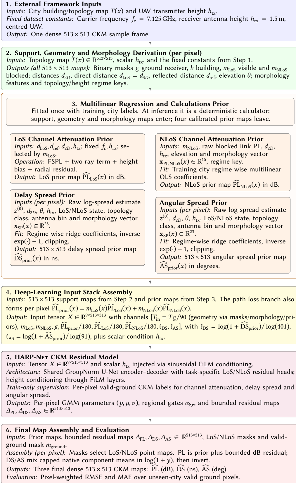
Figure 3.2: Detailed methodology data flow from external inputs to final assembled CKM maps, showing inputs, operations and outputs of each stage.
