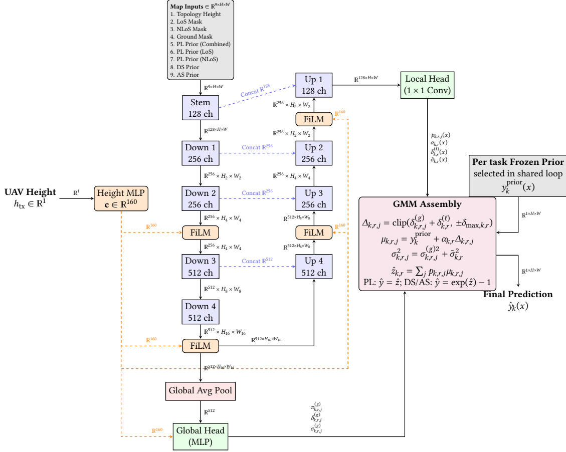
Figure 3.10: Schematic of the final large capacity shared UNet architecture with FiLM conditioning. The backbone and decode logic are shared, while each task uses its own heads and frozen prior.
