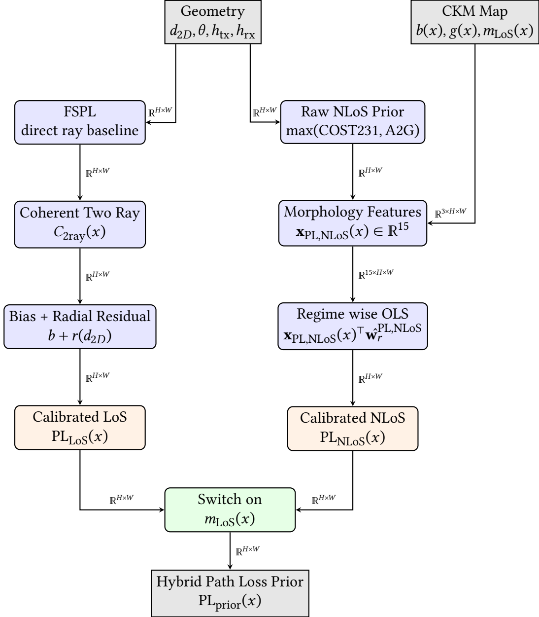
Figure 3.4: Pipeline for the hybrid path loss prior. The LoS branch uses an explicit two ray interference model, while the NLoS branch calibrates a raw prior against map derived morphology features using regime wise OLS. The two branches are hard switched by the LoS mask to produce the final frozen prior.
