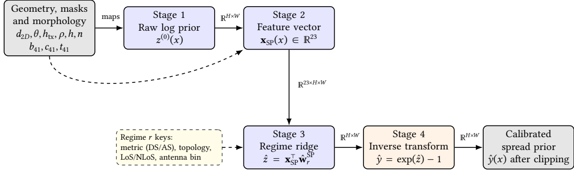
Figure 3.9: Pipeline for the delay and angular spread priors. Both spread modalities share this identical linear architecture, predicting expected spread in the log domain via regime wise ridge regression over 23 spatial and geometric features.
