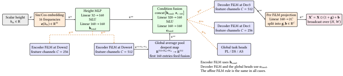
Figure 3.10: Detailed sinusoidal height conditioning path.
