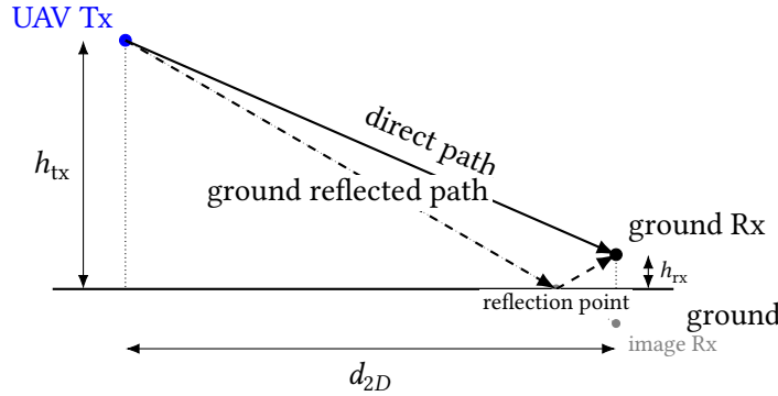
Figure 2.1: Direct and specular ground reflected paths in the two ray model.
