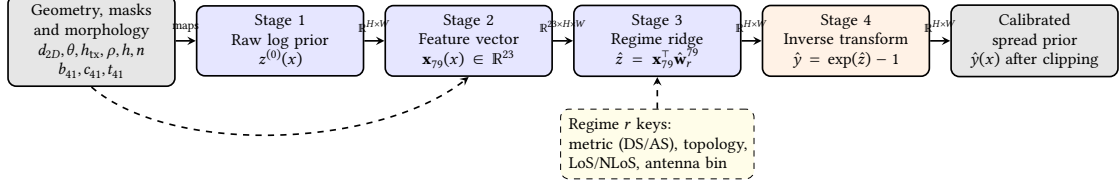
Figure 3.8: Pipeline for the delay and angular spread priors. Both spread modalities share this identical linear architecture, predicting expected spread in the log domain via regime wise ridge regression over 23 spatial and geometric features.
