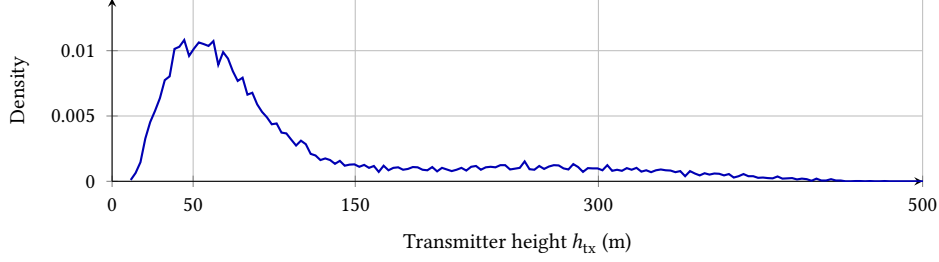
Figure 3.2: Empirical transmitter height density read directly from the CKM HDF5 database using the 3 m histogram of (3.3), linearly interpolated between bin centres for display. Most training support lies in the low and mid-altitude bands.
