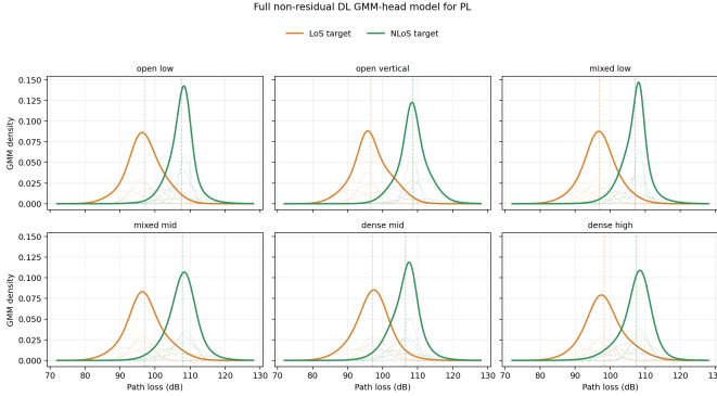
Fig. 6. Full non-residual DL GMM head model for path loss (PL): target GMM-5 fits by topology group. Thick curves show the summed LoS/NLoS mixture densities, faint dotted curves show the individual Gaussian components, and dashed vertical lines mark the marginal means. The diagnostic exposed different LoS/NLoS marginals and motivated distribution aware heads before returning to prior anchored residual learning.
