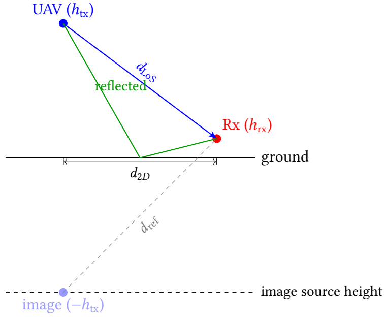
Figure D.1: Two ray geometry. Direct path (blue) has length d_{LoS} ; reflected path (green) has the same total length as the image source path (gray dashed), which is d_{ref} .
