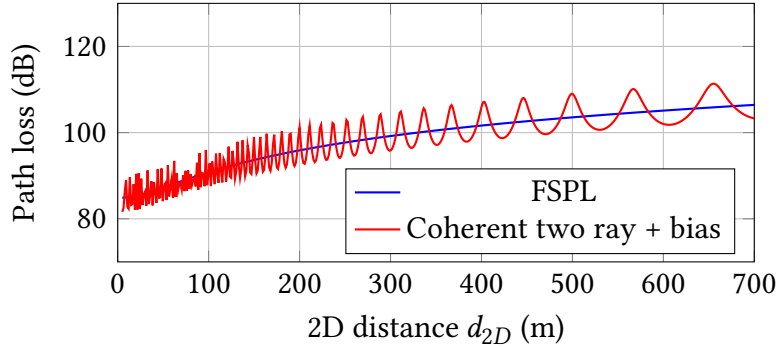
Figure 3.6: Schematic comparison of FSPL and the calibrated coherent two ray component for a 60 m UAV at 7.125 GHz ( h_{\text{tx}} = 1.5 m), zoomed to the 700 m near field that contains the full 513 \times 513 map diagonal. The plotted red curve uses the code loaded 60 m calibration values before adding the radial residual profile, so it shows the constructive/destructive interference term rather than the full final LoS prior.
