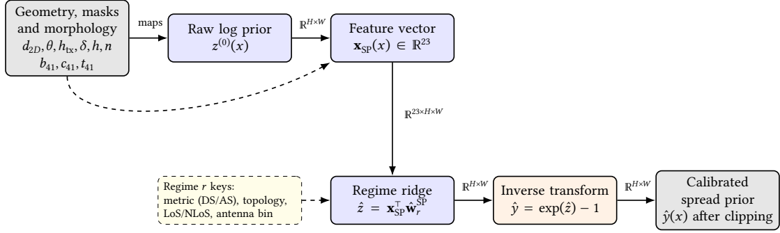
Figure 3.8: Pipeline for the delay and angular spread priors. Both spread modalities share this identical linear architecture, predicting expected spread in the log domain via regime wise ridge regression over 23 spatial and geometric features.
