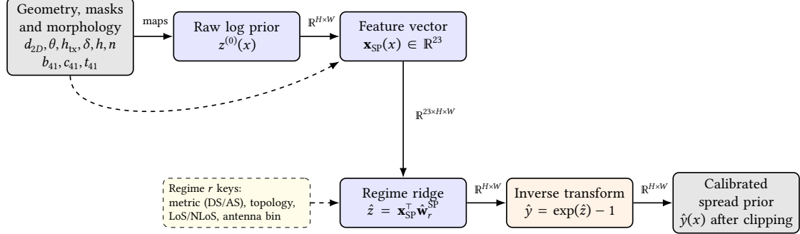
Figure 3.8: Pipeline for the delay and angular spread priors. Both spread modalities share this identical linear architecture, predicting expected spread in the log domain through ridge calibration by regime over 23 spatial and geometric features.
