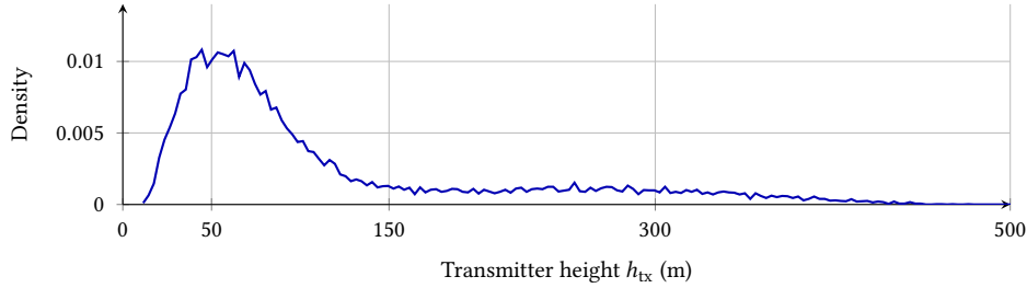
Figure 3.1: Empirical transmitter height density read directly from the CKM HDF5 database using the 3 m histogram of (3.3), linearly interpolated between bin centres for display. Most training support lies in the low and mid-altitude bands.
