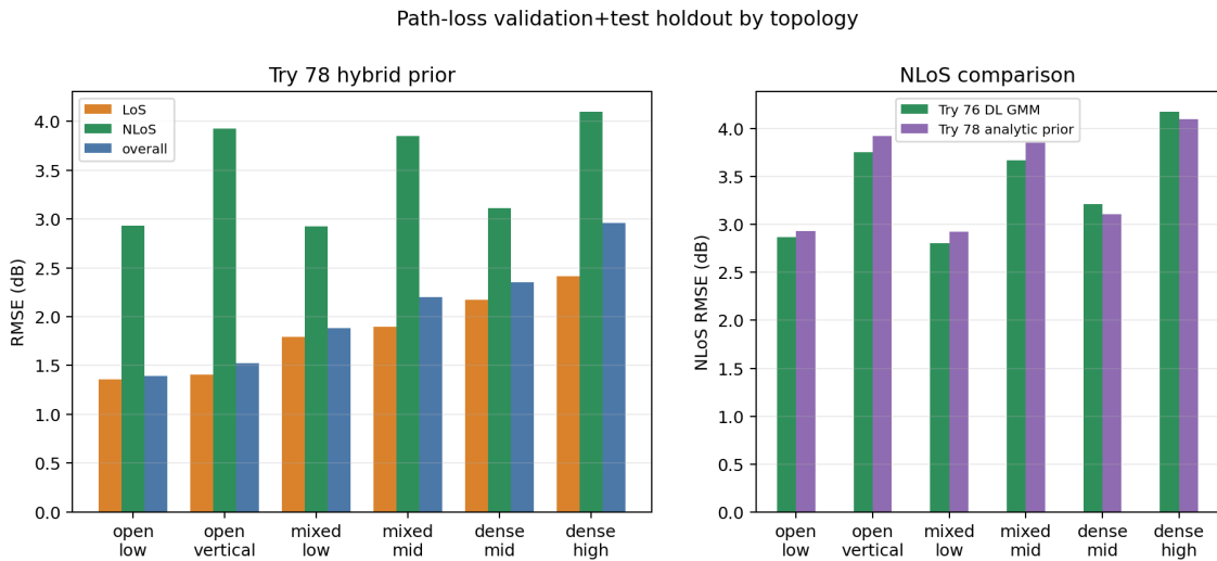
Figure 4.3: Path-loss prior by topology class. Left: LoS, NLoS and overall pixel-weighted RMSE for each of the six topology classes. The LoS RMSE grows monotonically with morphological density, mirroring the growth of the LoS target standard deviation reported for the distribution-first model in Table 4.6. Right: NLoS RMSE side by side with the distribution-first DL model on the same six topology classes. The two methods agree within roughly 1 dB per class, which is what reduces the choice between the two pipelines to deployability rather than accuracy.
