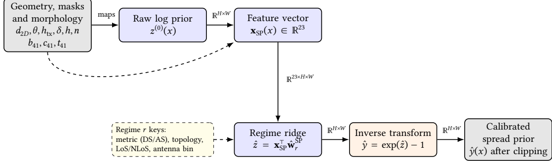
Figure 3.8: Pipeline for the delay and angular spread priors. Both spread modalities share this identical linear architecture, predicting expected spread in the log domain via regime wise ridge regression over 23 spatial and geometric features.
