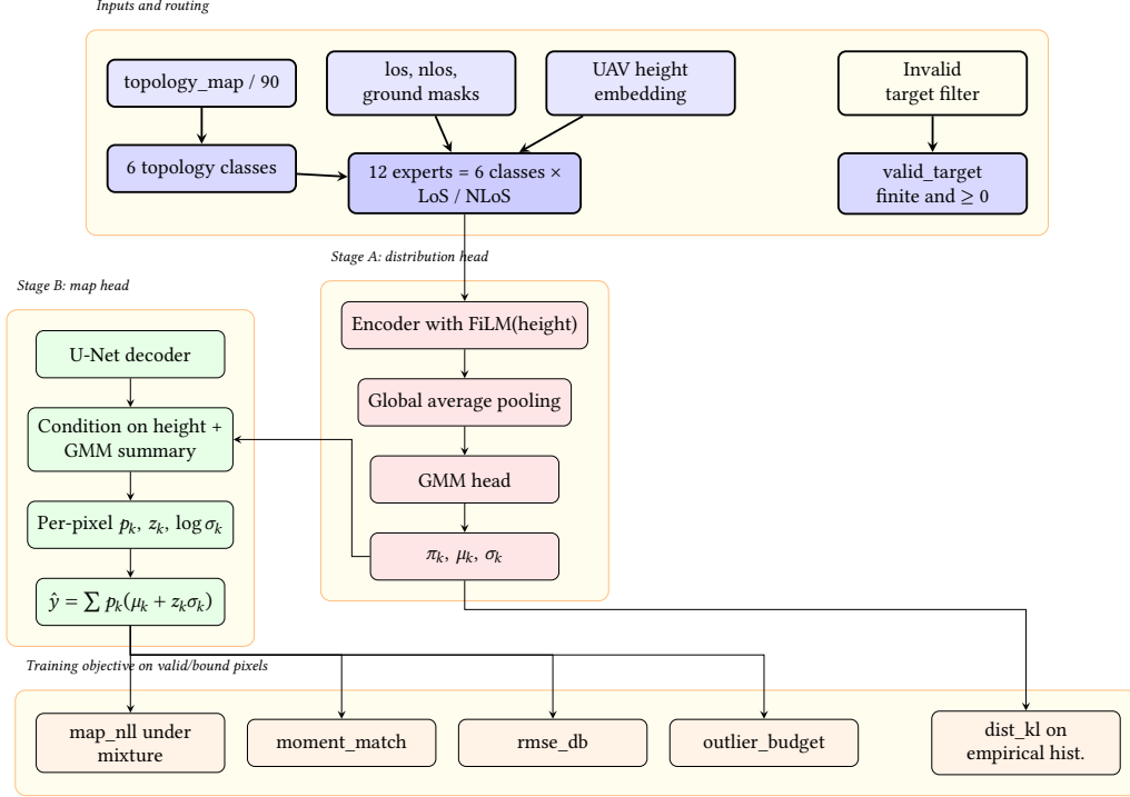
Figure 3.2: Distribution-first path-loss system. Stage A learns global GMM parameters (\pi_k, \mu_k, \sigma_k) from pooled features conditioned on UAV height; Stage B produces per-pixel soft assignments and within-component offsets anchored to those parameters.
