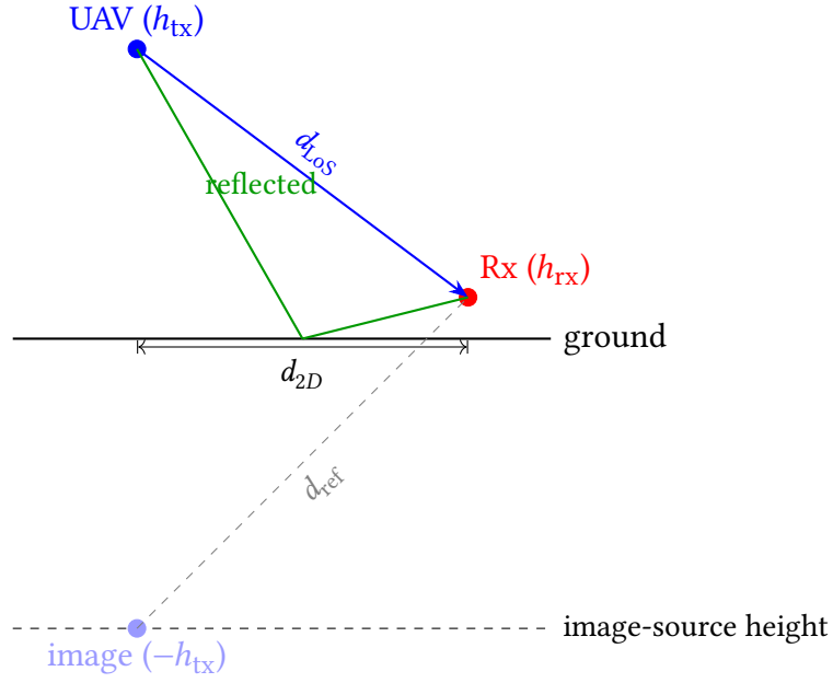
Figure 3.4: Two-ray geometry. Direct path (blue) has length d_{LoS} ; reflected path (green) has the same total length as the image-source path (gray dashed), which is d_{ref} .
