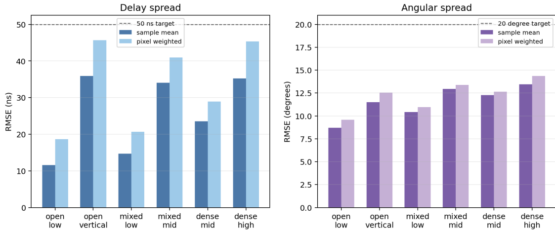
Figure 4.2: Distribution-first spread DirectML test RMSE per expert, separated by spread target. For each topology class, paired bars show sample-mean and pixel-weighted aggregation. Dashed grey lines mark the original project targets (50 ns for delay spread, 20^\circ for angular spread). The angular-spread experts beat the target across all topology classes; the delay-spread experts also remain below 50 ns, but their pixel-weighted errors are larger and less competitive with the final ridge calibration.
