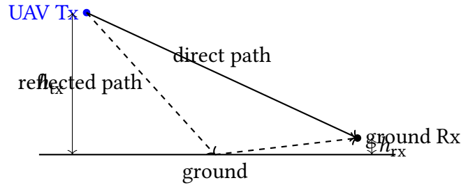
Figure 2.1: Direct and ground-reflected paths in the two-ray model.
