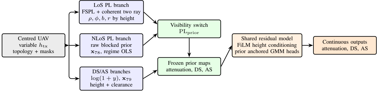
Fig. 2. Compact prior anchored pipeline used for the reported final system. The transmitter is always centred, but its height varies by sample. Frozen height aware priors are produced first and then used as channels for the final prior anchored residual GMM model.
