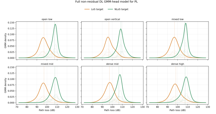
Fig. 6. Full non residual DL GMM head model for channel attenuation (PL/path_loss): target GMM-5 fits by topology group. Thick curves show the summed LoS/NLoS mixture densities, faint dotted curves show the individual Gaussian components, and dashed vertical lines mark the marginal means. The diagnostic exposed different LoS/NLoS marginals and motivated distribution aware heads before returning to prior anchored residual learning.
