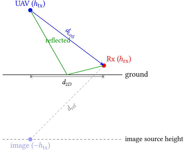
Figure 3.3: Two ray geometry. Direct path (blue) has length d_{LoS} ; reflected path (green) has the same total length as the image source path (gray dashed), which is d_{ref} .
