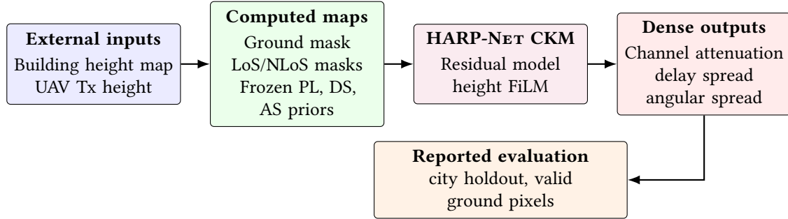
Figure 3.2: High level methodology flow. The user supplies the city height map and transmitter height. The pipeline constructs support masks and frozen prior maps, then HARP-NET CKM predicts residual corrections for the three CKM outputs.
