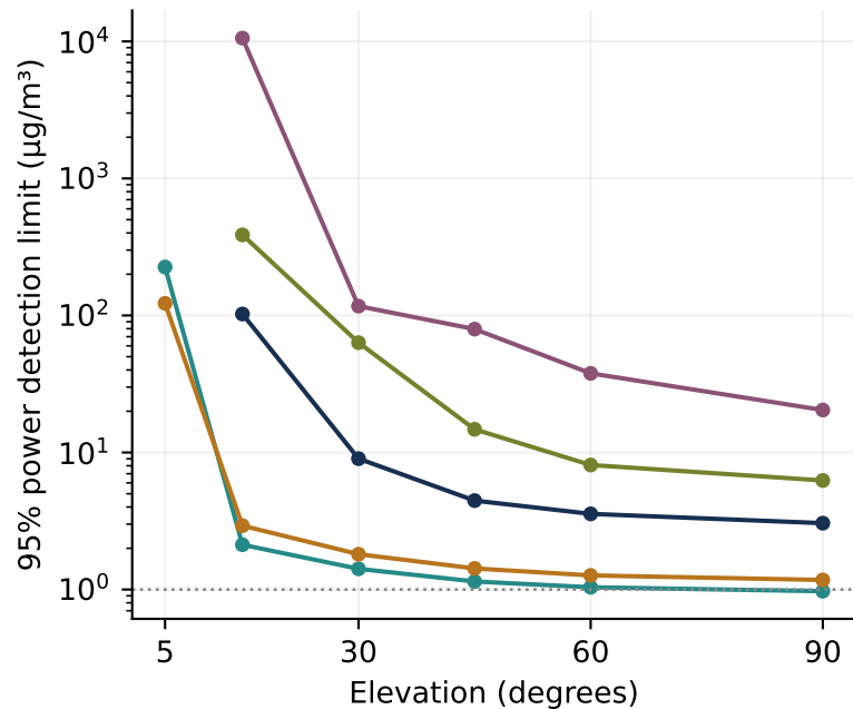
Formaldehyde
