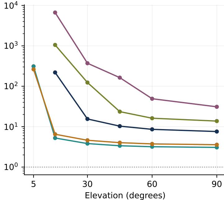
Methanol
