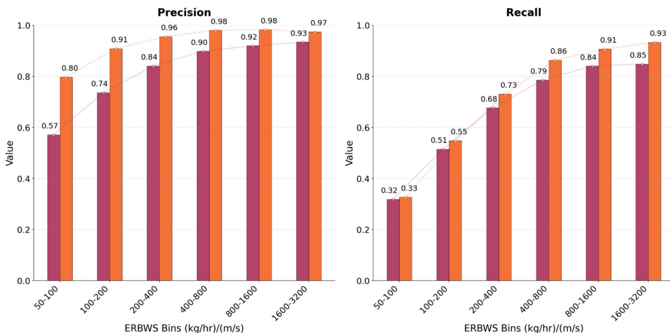
Fig. 1. MAPL-EMIT exhibits high precision and recall across plumes with a wide range of emission rates on the synthetic plume test split. Precision (Left panel) and recall (Right panel) are binned for different plume intensity levels, defined as emission rate (kg/h) divided by 10 m elevation wind speed (m/s) (ERBWS), for scenes with single plumes (orange) as well as for multiple overlapping plumes (in the same EMIT tile) (magenta). The numbers above the bars indicate the precision and recall for each ERBWS bin.
