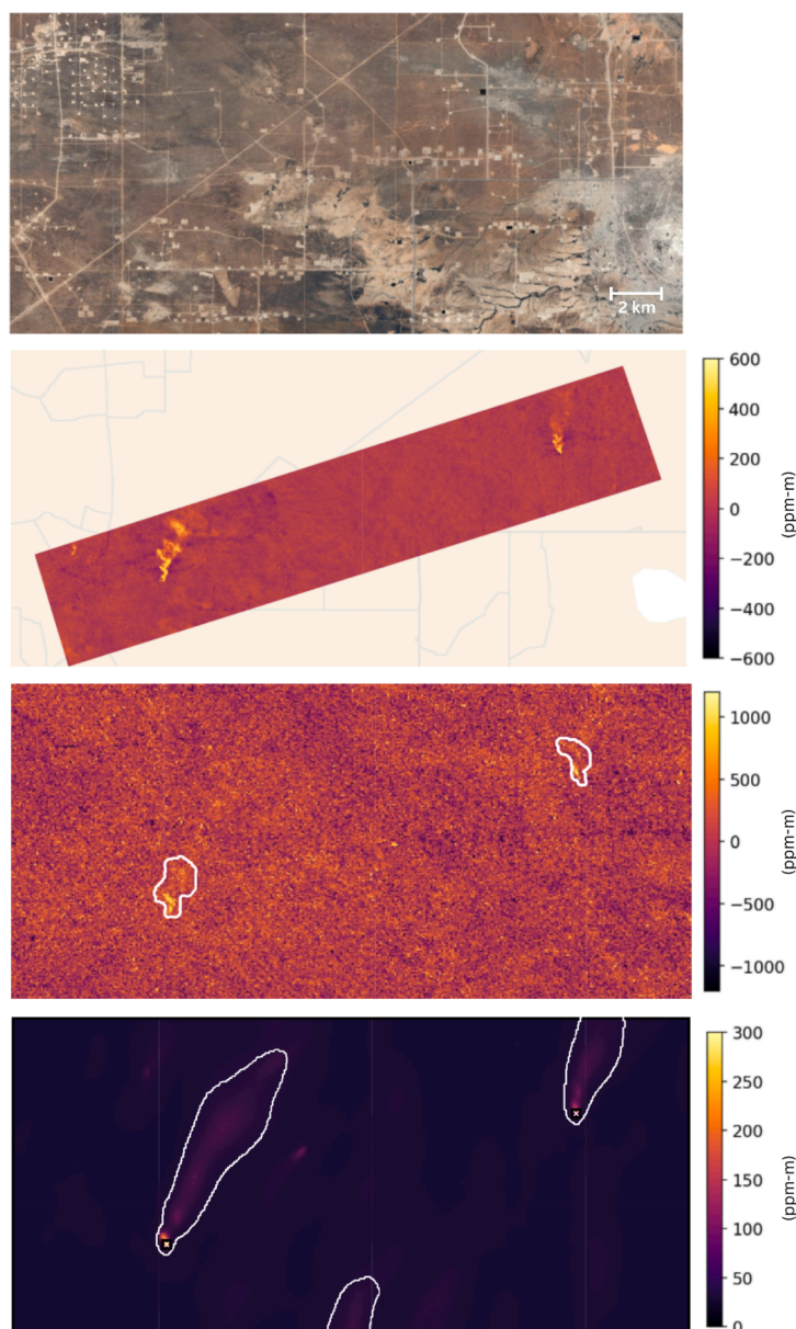
Fig. 4. Enhanced signal-to-noise ratio and verification of MAPL-EMIT plumes against high-resolution aerial enhancements from AVIRIS-3. The panels display (from Top to Bottom ): RGB, coincident AVIRIS-3 airborne observations resampled to 60 m resolution, NASA L2B enhancement with identified plume complexes on Top , where plumes are hard to distinguish from background noise, and MAPL-EMIT enhancements and plumes, which successfully suppress surface artifacts and accurately predict plume morphologies aligned with AVIRIS-3 observations.
