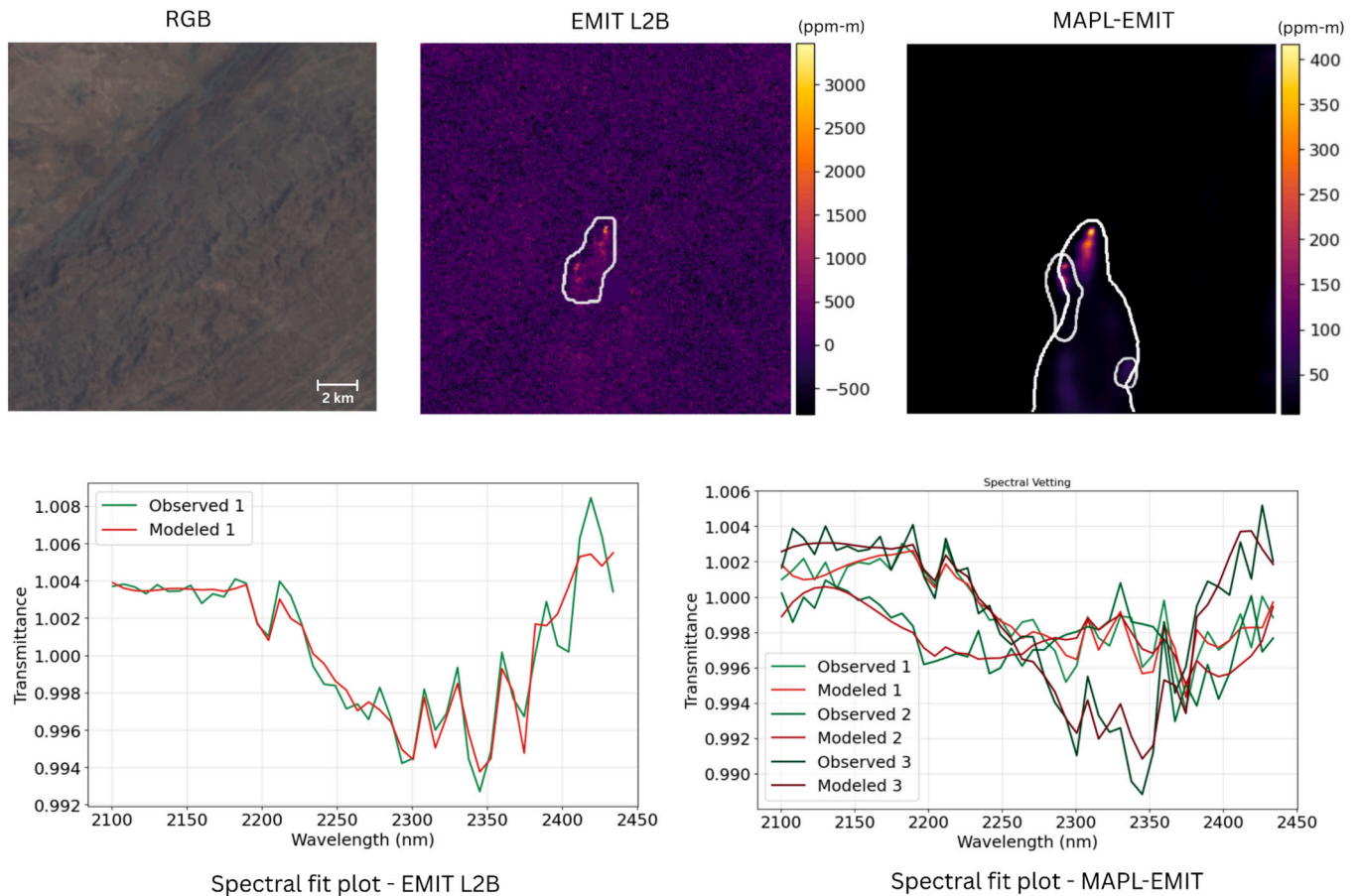
Fig. 2. MAPL-EMIT detection and disambiguation of overlapping methane plumes. (Top row) RGB (Left), NASA L2B enhancements with plume masks (Middle), and MAPL-EMIT enhancements with plume delineation (Right). (Bottom row) Spectral fits provide physical verification. Observed transmittance ratios align with modeled methane absorption manifolds, supporting plume authenticity. While the first MAPL-EMIT plume shows a robust spectral fit, the second appears less definitive, likely due to its weaker intensity.
