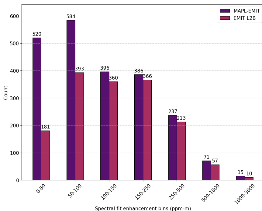
Fig. 3. MAPL-EMIT identifies more potential plumes than the official EMIT L2B plume complexes. Plumes are binned by spectral fit enhancement ( Methods ). MAPL-EMIT (purple) consistently identifies more plumes across all intensities, specifically more than 2× the number of detections for the 0 to 50 ppm-m bin. The numbers above the bars indicate the number of identified plumes in each enhancement bin.
