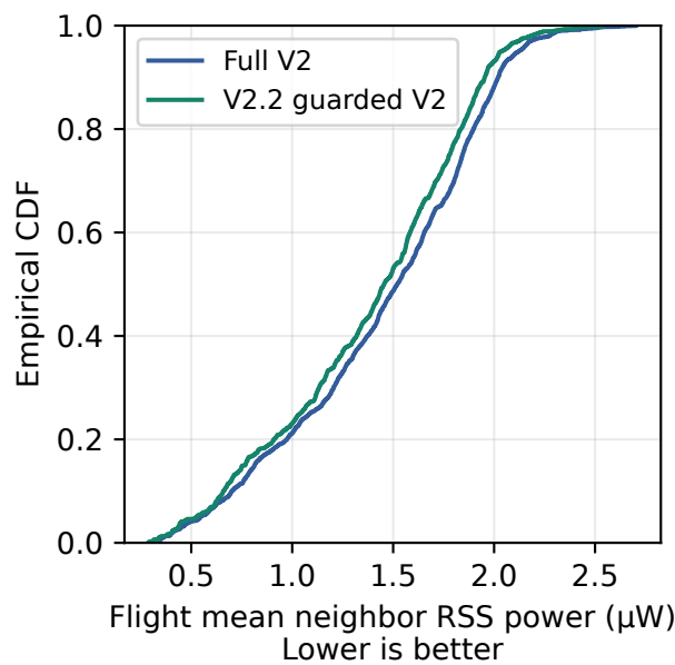
Standard fresh routes: 500 routes \times 5 fixed policy seeds CDFs use 2331 common successful pairs; bars include all 2,500 flights per controller
