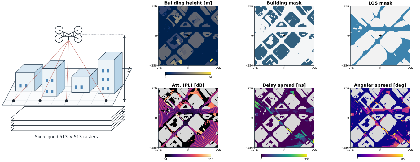
Fig. 1. One Barcelona realization (sample_02806) at h_{tx} = 69.4 m. The left illustration shows an elevated UAV base station serving ground receivers above six aligned 513 \times 513 rasters. The panels show building height, building mask, LOS, attenuation, delay spread, and angular spread. Crosses mark the centered transmitter; gray areas are building pixels excluded from the metrics. For this sample, the stored three- and six-class labels are dense_highrise and dense_block_midrise .
