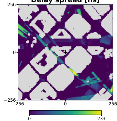
Delay spread [ns]
