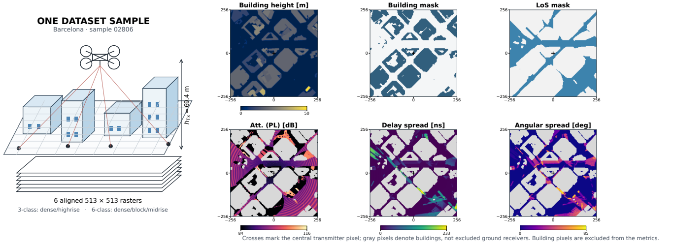
Fig. 1. One released Barcelona realization at h_{tx} = 69.4 m. The left schematic separates transmitter height from the six co-registered rasters; the panels show the stored building height, building mask, LoS, attenuation, delay spread, and angular spread. Crosses mark the centered transmitter. Gray pixels denote buildings, not excluded ground receivers; building pixels are excluded from the metrics.
