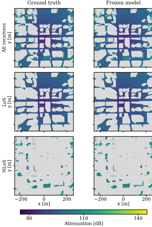
Fig. 3. Held-out Vancouver sample_15262 ( h_{tx} = 50.30 m; urban, low-height regime). Columns compare RT ground truth with the frozen model; rows show all valid receivers, LoS, and NLoS. Gray marks buildings in the first row and receivers outside the displayed visibility subset below; building pixels never enter the metrics. The map has 119180 LoS and 25607 NLoS receivers, with 2.10 and 2.53 dB RMSE.
