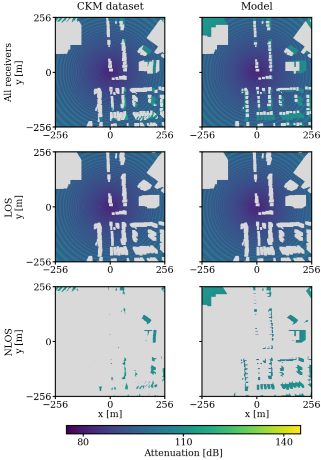
Fig. 3. Held-out Vancouver sample_15142 ( h_{tx} = 52.22 m; suburban, low-transmitter regime). The dataset column shows only stored valid targets, while the model column predicts every ground receiver. Thus, gray in the first dataset panel denotes buildings or an unavailable target; in the first model panel it denotes buildings only. Lower rows additionally exclude the other visibility class. Metrics use valid targets only. The map has 198083 LOS and 12614 NLOS targets; full, LOS, and NLOS RMSE are 1.85, 1.60, and 4.11 dB.
