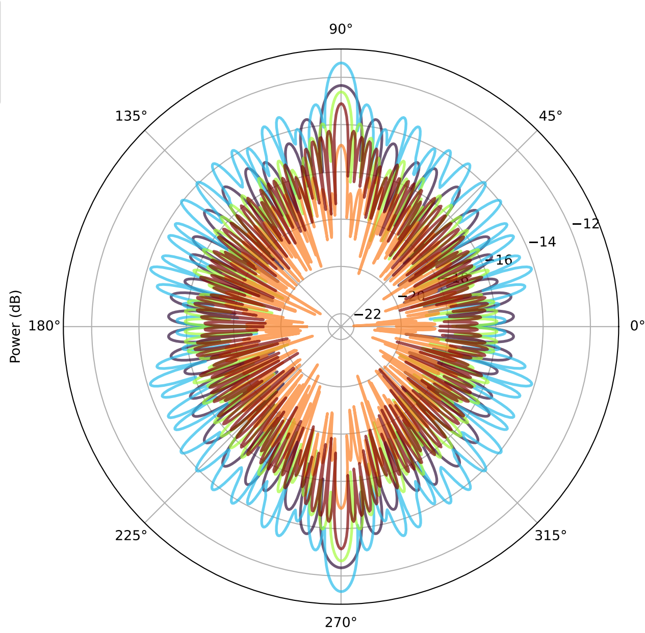
XY Plane Radiation Pattern
