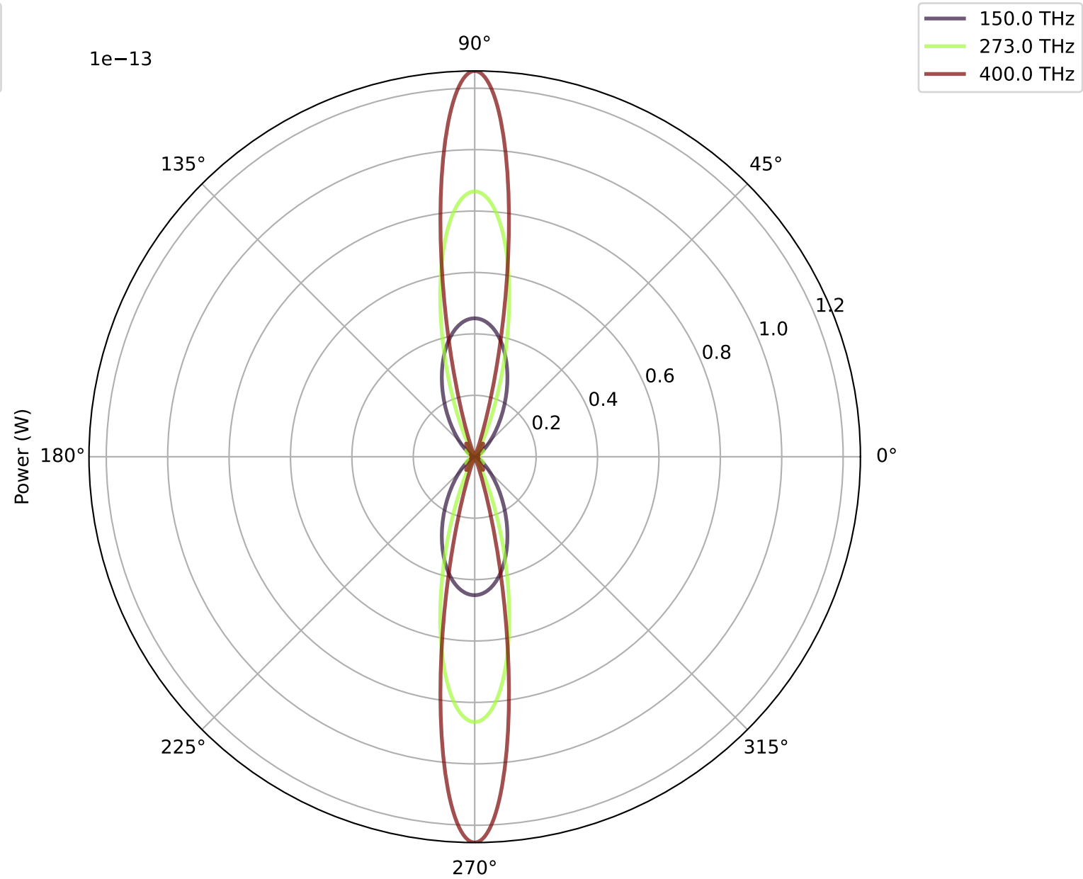
YZ Plane Radiation Pattern
