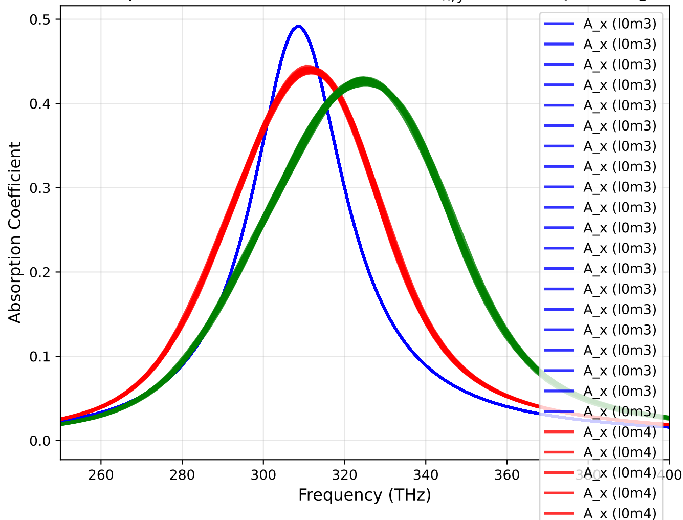
Absorption Coefficient - No Disorder ( \sigma_{x,y} = 0 nm, \sigma_{\theta} = 0 deg)
