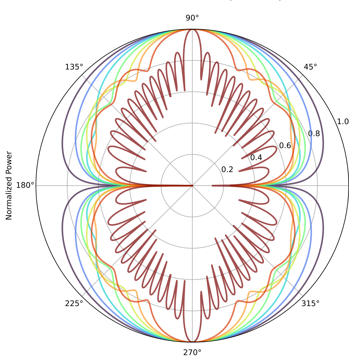
XZ Plane Radiation Pattern (219.7 THz)
