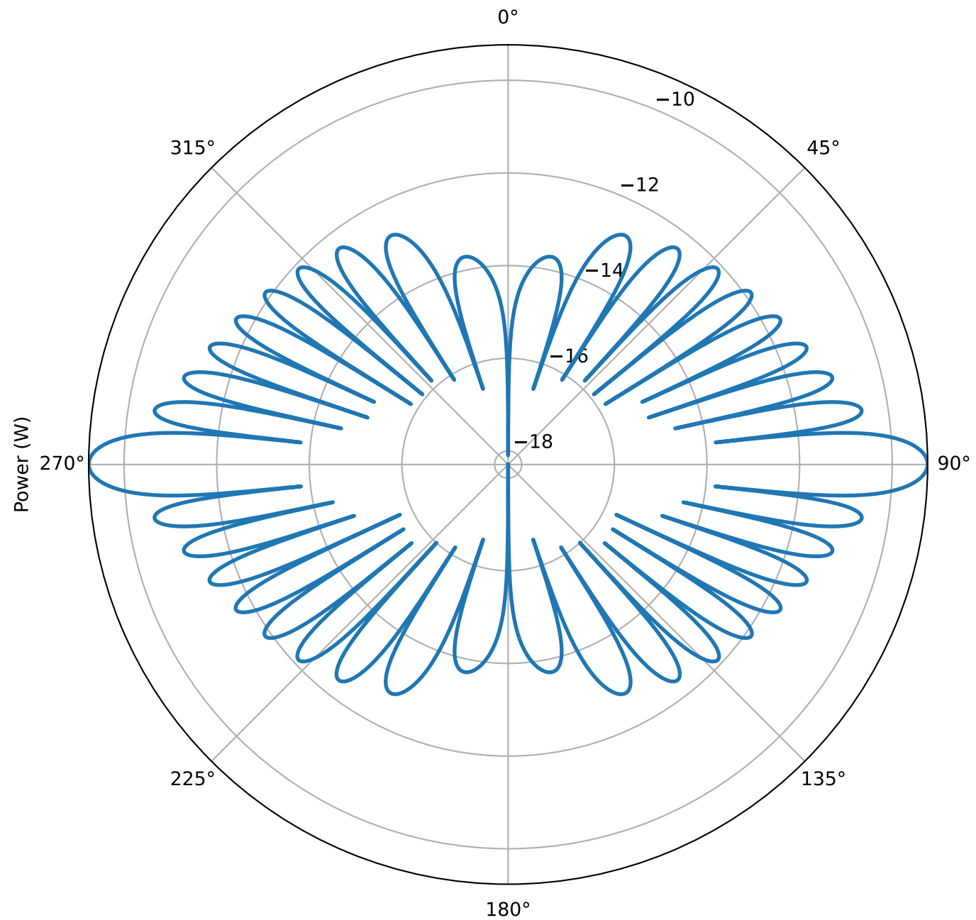
Radiation Pattern at 166.4 THz
