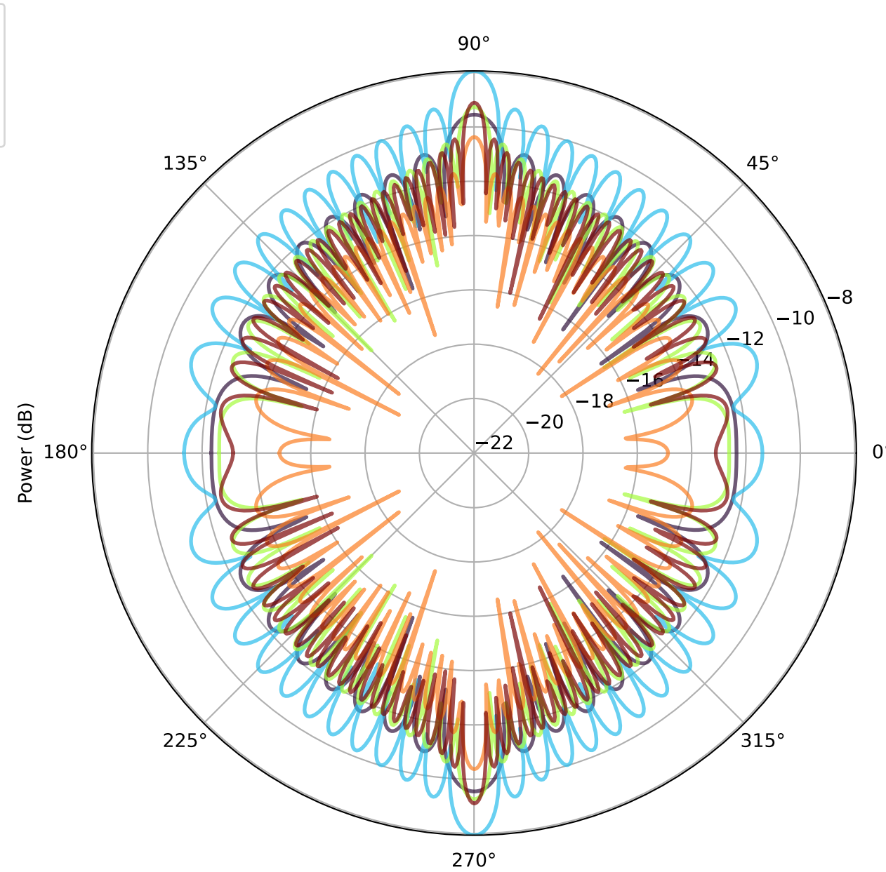
YZ Plane Radiation Pattern
