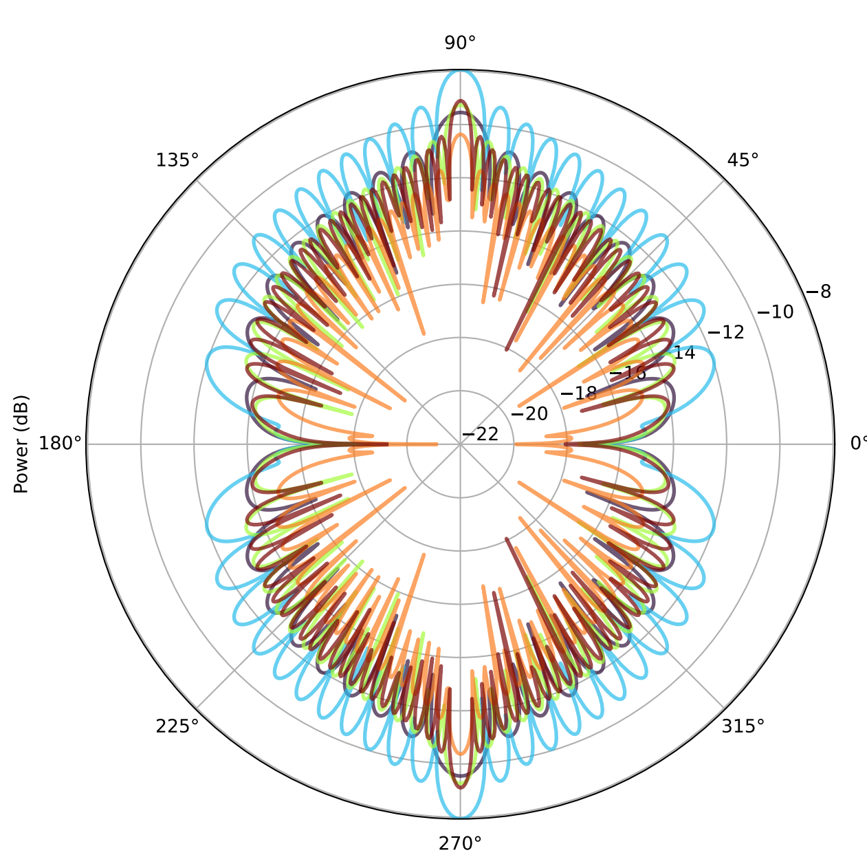
XZ Plane Radiation Pattern
