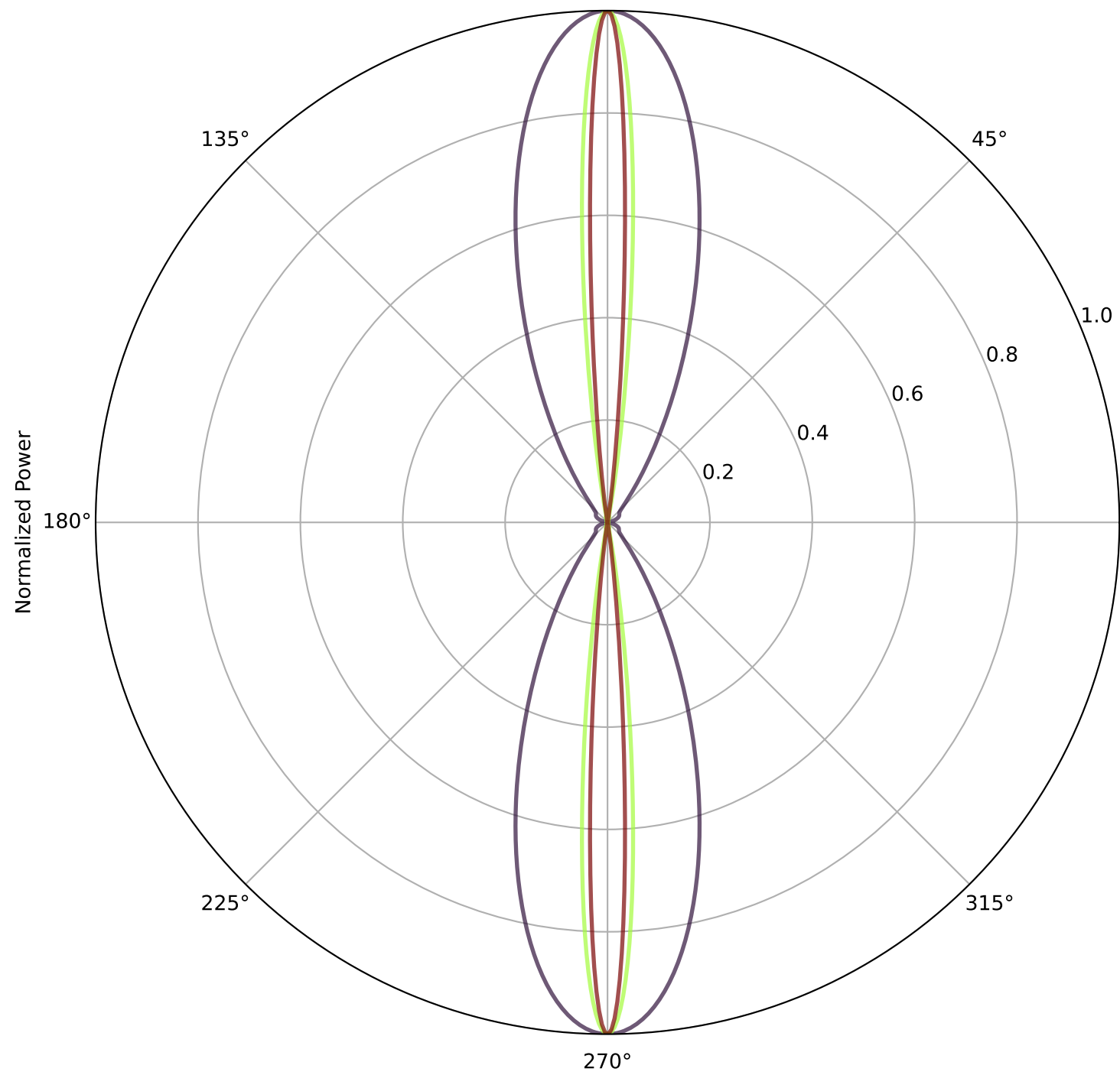
XZ Plane Radiation Pattern (linear)
