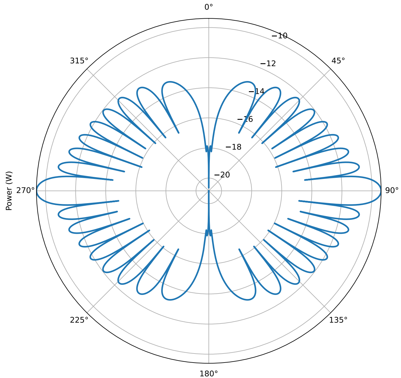
Radiation Pattern at 158.2 THz
