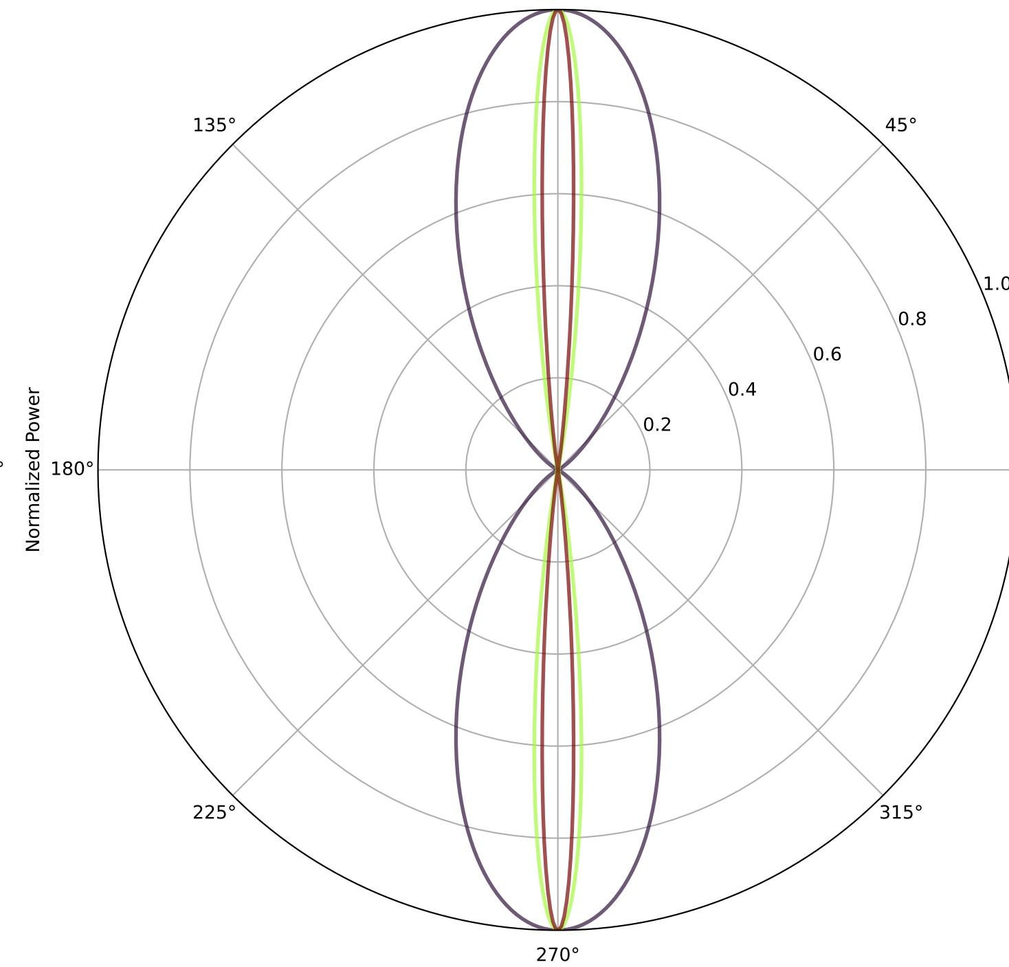
YZ Plane Radiation Pattern (linear)
