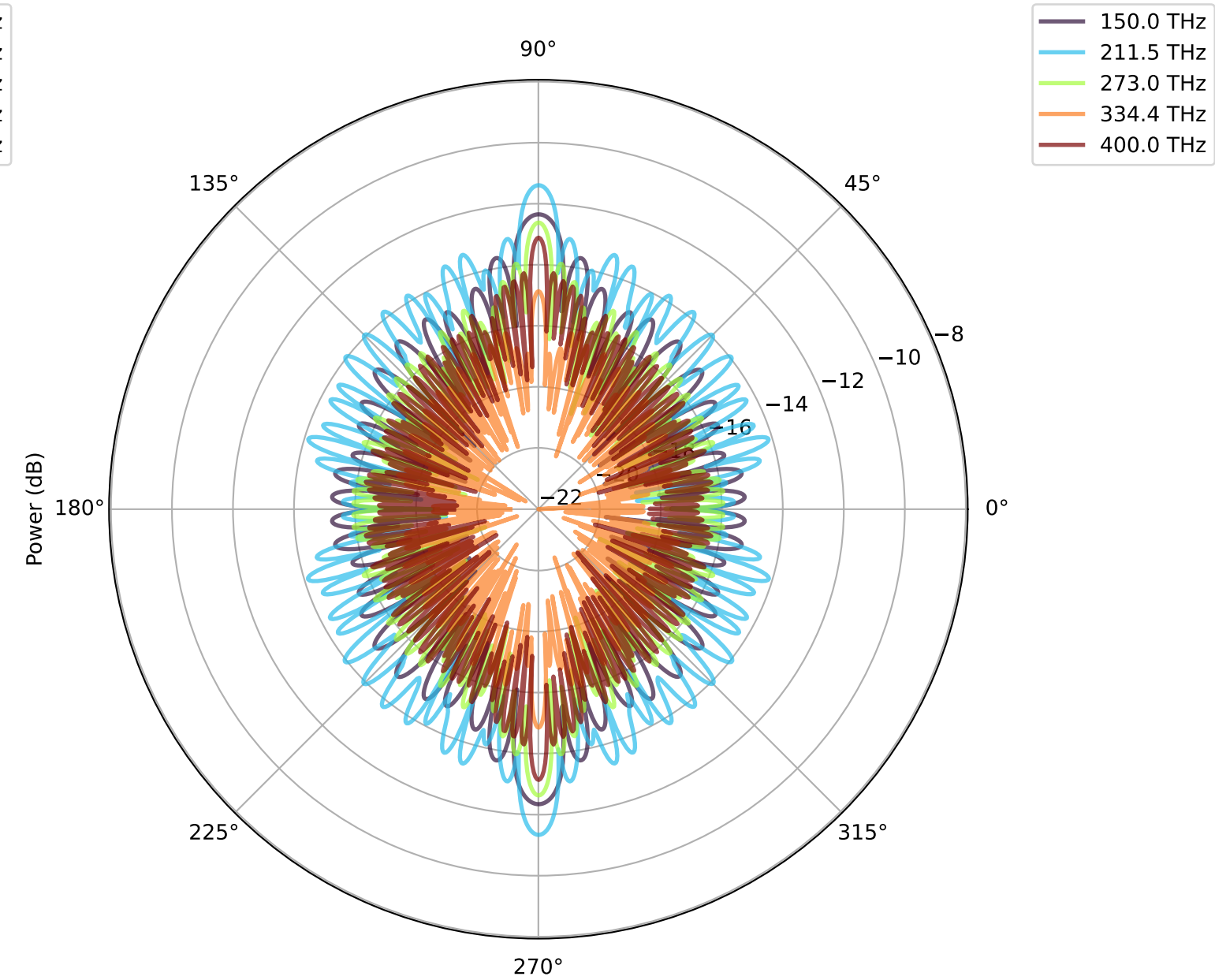
XY Plane Radiation Pattern
