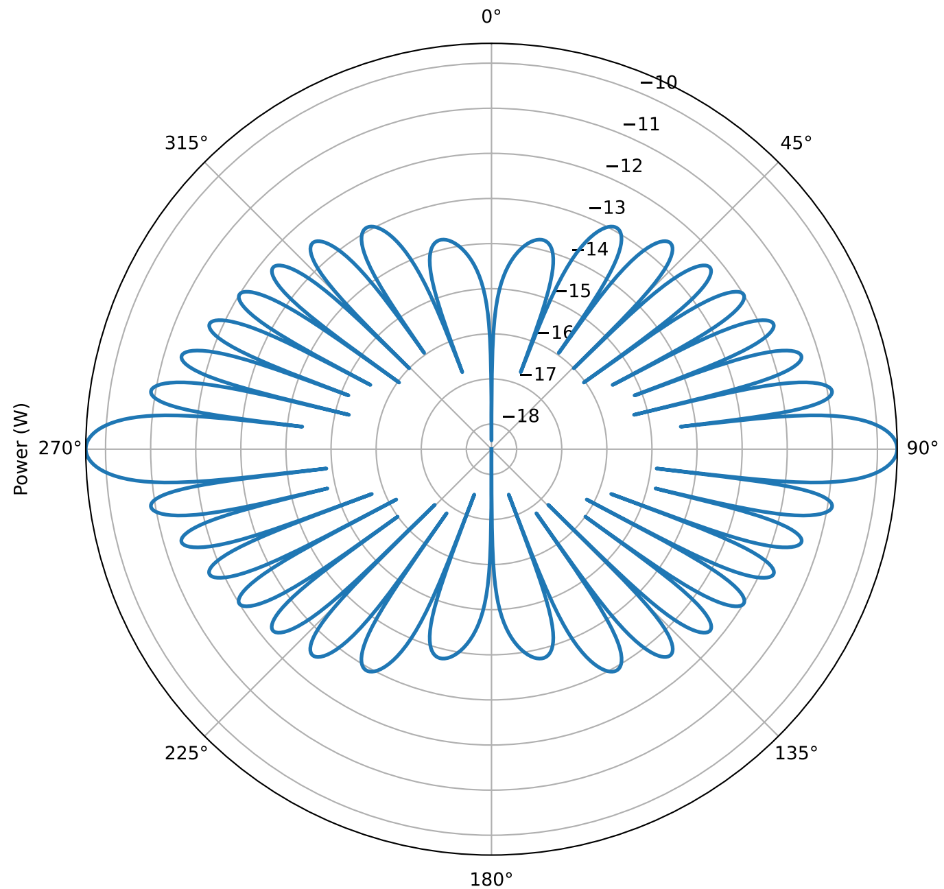
Radiation Pattern at 150.0 THz
