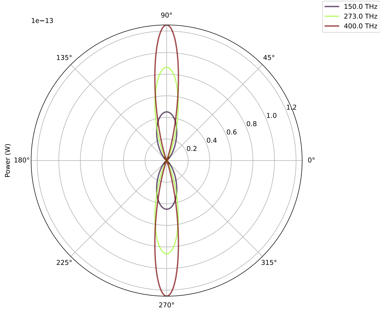
XZ Plane Radiation Pattern
