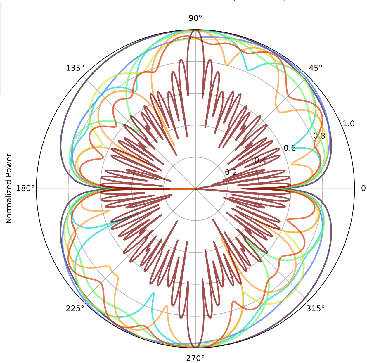
XY Plane Radiation Pattern (219.7 THz)
