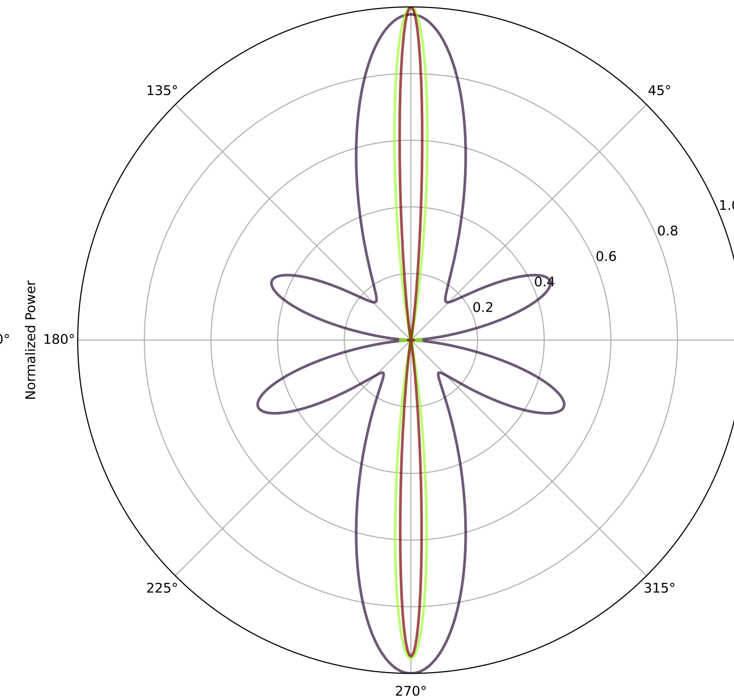
XY Plane Radiation Pattern (linear)
