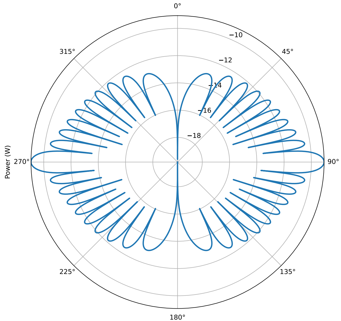
Radiation Pattern at 174.6 THz
