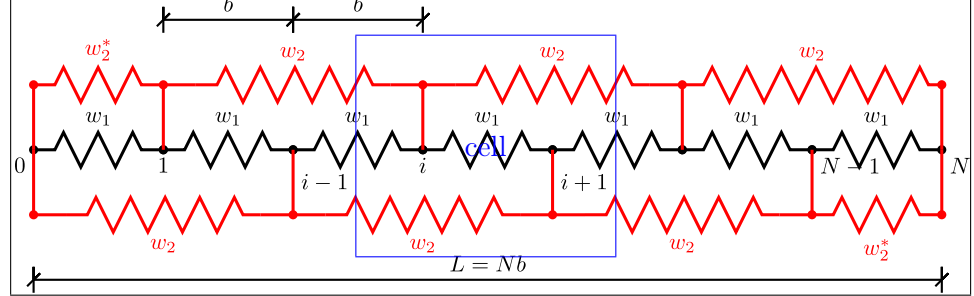
Figure 3.23: 1D arrangement of non-linear springs with connections to (a) next-to-neighbour node (Combesure 2022, Fig. 3(a)). The blue box is one micro-cell of one period, width 2b , containing an odd and an even i .
