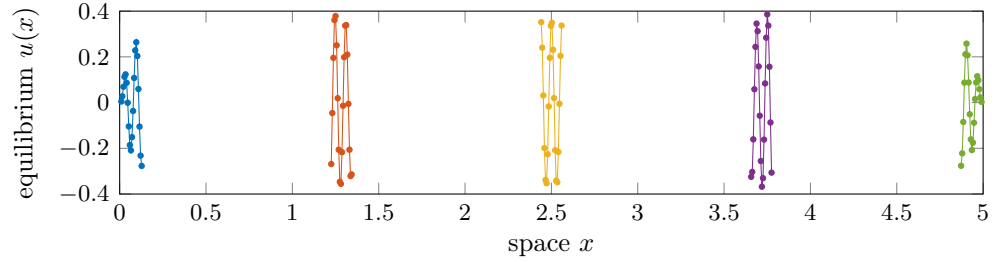
Figure 3.35: an equilibrium of the heterogeneous Swift–Hohenberg PDE determined by the patch scheme
