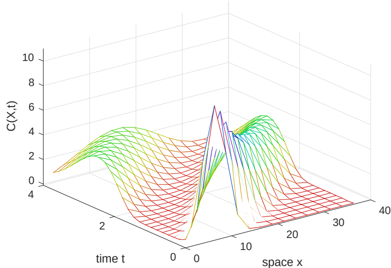
Figure 6.3: macro-scale view of heterogeneous advection-diffusion PDE along a (periodic) channel obtained via the patch scheme.
