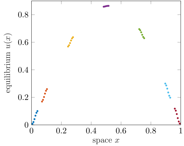
Figure 3.17: Equilibrium of the heterogeneous diffusion problem with forcing the same as that applied at time t = 1 , and for relatively large \epsilon = 0.04 so we can see the patches. By default this code sets \epsilon = 0.004 whence the microscale heterogeneity and patches are tiny.
