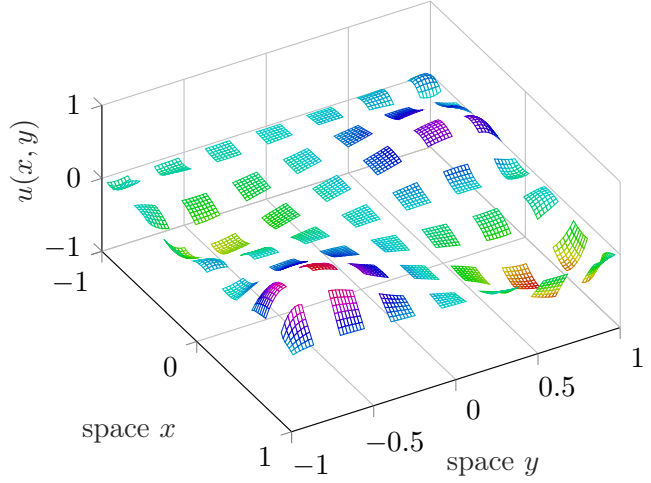
Figure 4.6: Equilibrium of the multiscale diffusion problem of Freese with Dirichlet zero-value boundary conditions (Section 4.5). The patch size is not small so we can see the patches and the sub-patch grid. The solution u(x, y) is boringly smooth.
