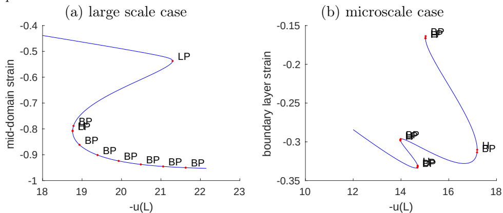
Figure 3.27: cross-sections through Figures 3.16 and 3.18: (a) large scale case, at the mid-point in space of Figure 3.18; (b) microscale case, in a boundary layer of Figure 3.16. These cross-sections are labelled with the various critical points.
