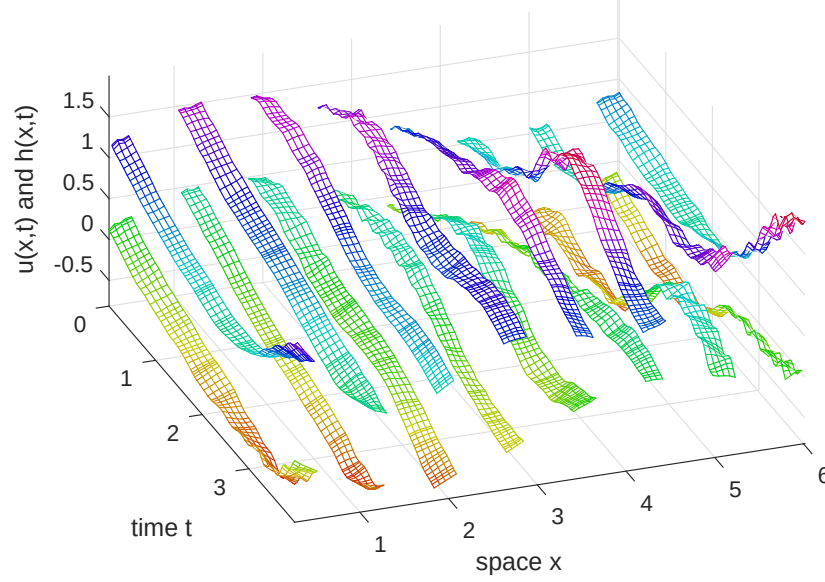
Figure 3.12: water depth h(x, t) (above) and velocity field u(x, t) (below) of the gap-tooth scheme applied to the Smagorinski shallow water wave PDEs ???. The microscale random initial component decays where the water speed is non-zero due to ‘turbulent’ dissipation.
