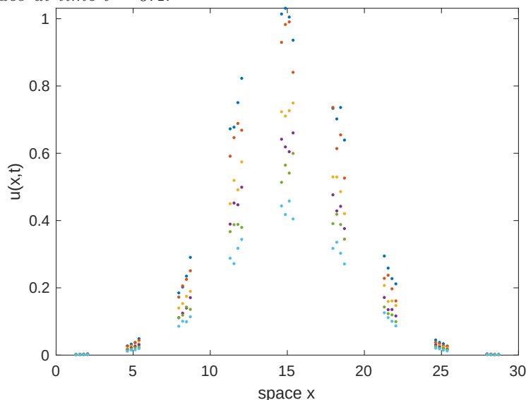
Figure 6.6: initial field u(x, y, z, 0) of the patch scheme applied to a heterogeneous diffusion PDE. The vertical spread indicates the extent of the structure in u in the cross-section variables y, z . Figure 6.7 plots the nearly smooth field values at time t = 0.4 .
