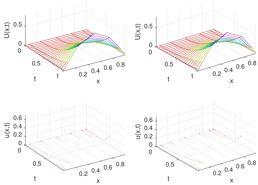
Figure 3.20: diffusion field u(x, t) of the patch scheme applied to the forced space-time heterogeneous diffusive (3.4). Simulate for seven patches (with a ‘Chebyshev’ distribution): the top stereo pair is a mesh plot of a macroscale value at the centre of each spatial patch at each projective integration time-step; the bottom stereo pair shows the corresponding tiny space-time patches in which microscale computations were carried out.
