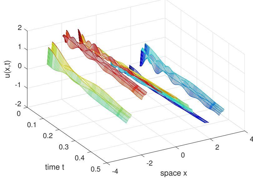
Figure 3.14: wave field u(x,t) of the gap-tooth scheme applied to the weakly damped wave ???. Over this shorter meso-time we see the macroscale wave emerging from the damped sub-patch fast waves.
