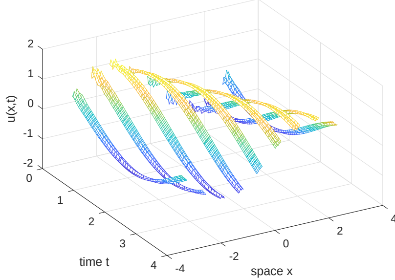
Figure 3.15: wave field u(x,t) of the gap-tooth scheme applied to the wave ?? . The microscale random component to the initial condition, the sub-patch fluctuations, decays, leaving the emergent macroscale wave in the heterogeneous media. This simulation uses nine patches of ‘large’ size ratio 0.25 for visibility.
