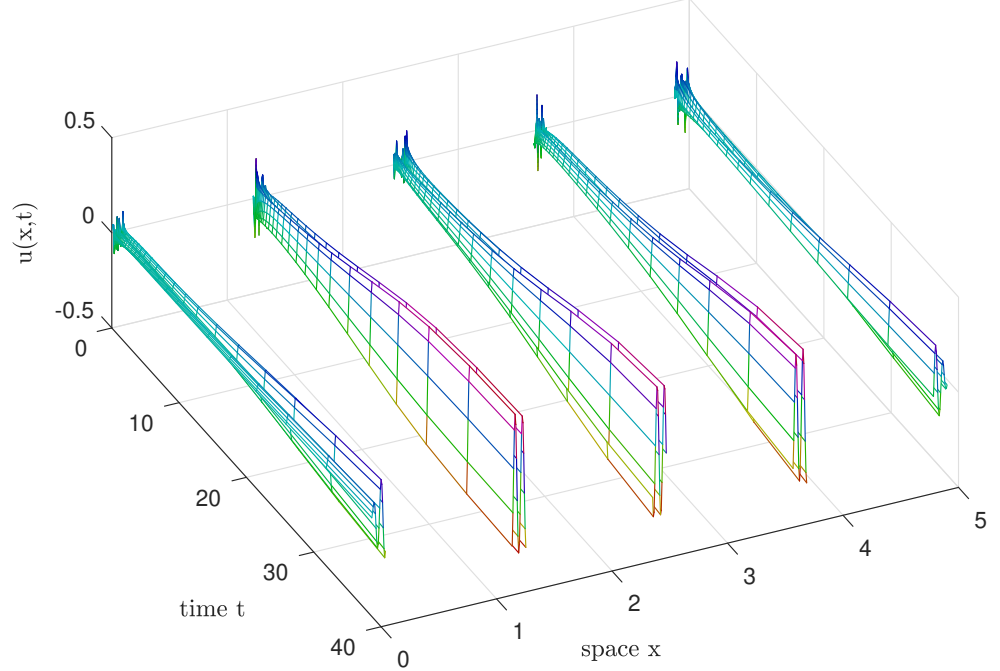
Figure 3.31: the field u(x,t) in the patch (gap-tooth) scheme applied to microscale heterogeneous Swift–Hohenberg PDE (Section 3.14). The heterogeneous coefficients are approximately uniform over [0.9, 1.1] . This heterogeneity has no noticeable affect on the simulation.
