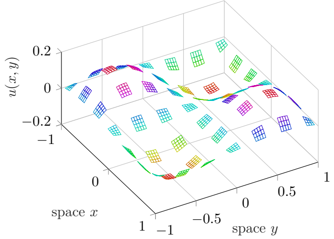
Figure 4.5: Equilibrium of the macroscale diffusion problem of Freese with Dirichlet zero-value boundary conditions (Section 4.4). The patch size is not small so we can see the patches.
