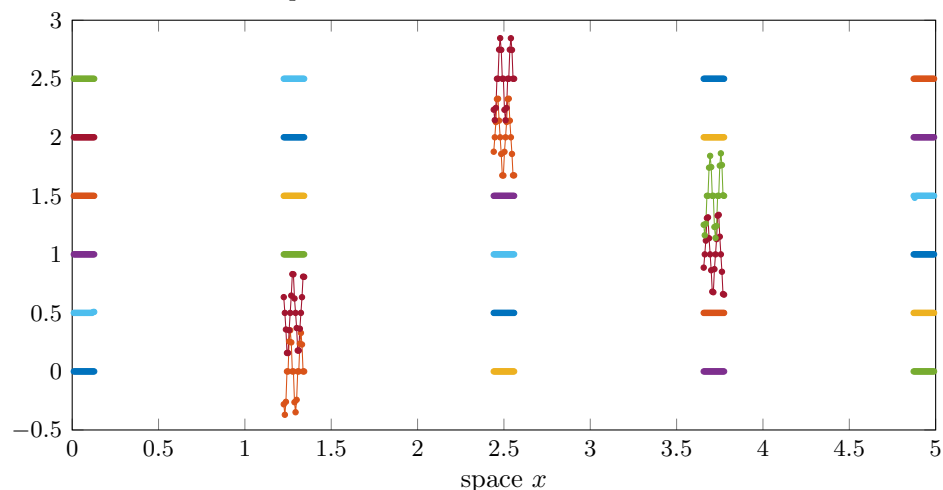
Figure 3.33: sparse approximations of the eigenvectors of the six slow modes of Figure 3.24. Plotted are sparse basis vectors for the invariant space spanned by the six slow eigenvectors: each basis vector shifted vertically to separate. Thus a fair approximation is that there are effectively two modes for each of the N - 2 = 3 interior patches.
