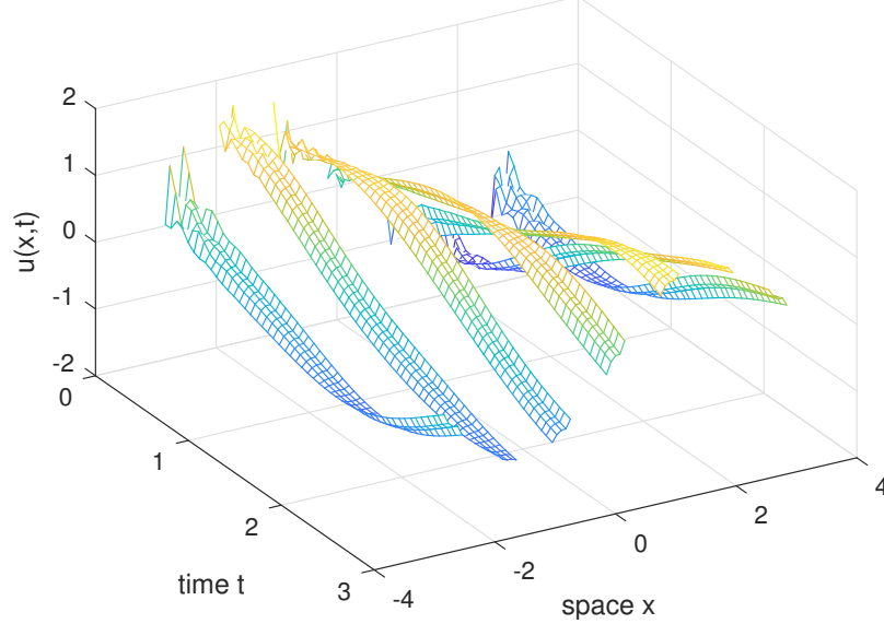
Figure 3.13: wave field u(x,t) of the gap-tooth scheme applied to the weakly damped wave ???. The microscale random component to the initial condition persists in the simulation until the weak damping smooths the sub-patch fluctuations—but the macroscale wave still propagates.
