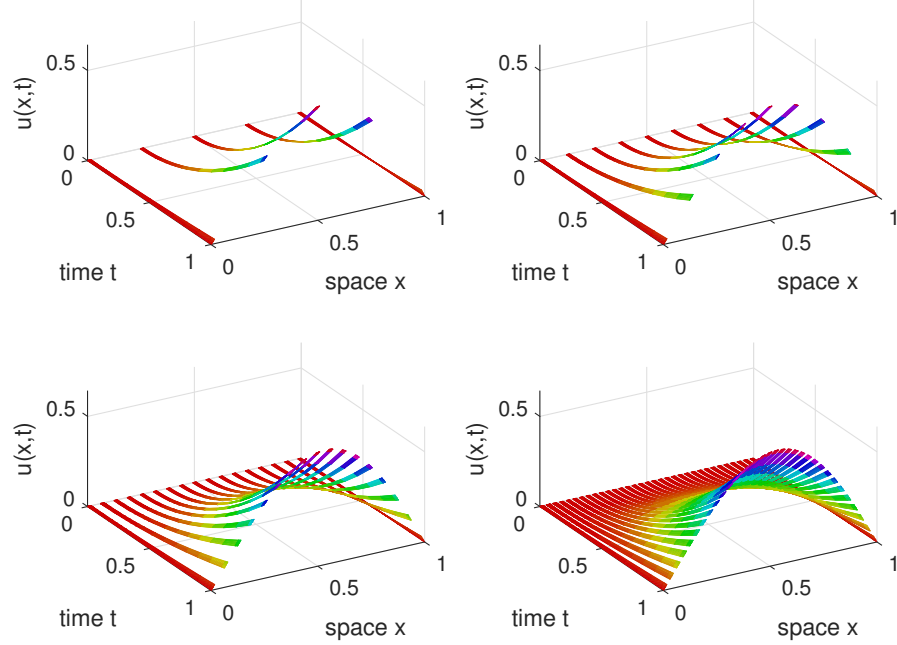
Figure 3.16: diffusion field u(x,t) of the patch scheme applied to the forced heterogeneous diffusive (3.3). Simulate for 5, 9, 17, 33 patches and compare to the full-domain simulation (65 patches, not shown).
