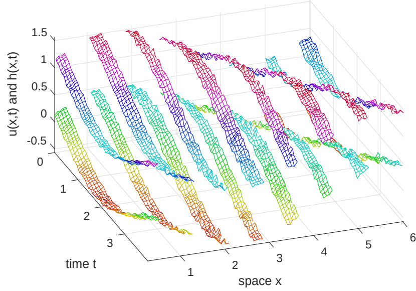
Figure 3.11: water depth h(x, t) (above) and velocity field u(x, t) (below) of the gap-tooth scheme applied to the ideal linear wave PDE ?? with f_1 = f_2 = 0 . The microscale random component to the initial condition persists in the simulation—but the macroscale wave still propagates.
