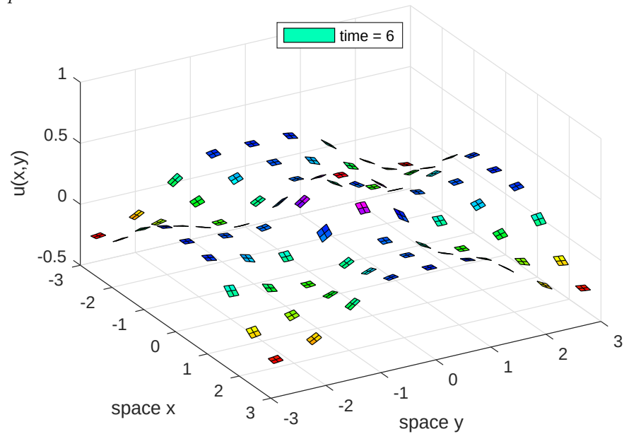
Figure 4.4: field u(x, y, t) at time t = 6 of the patch scheme applied to the simple wave PDE with initial condition in ??.
