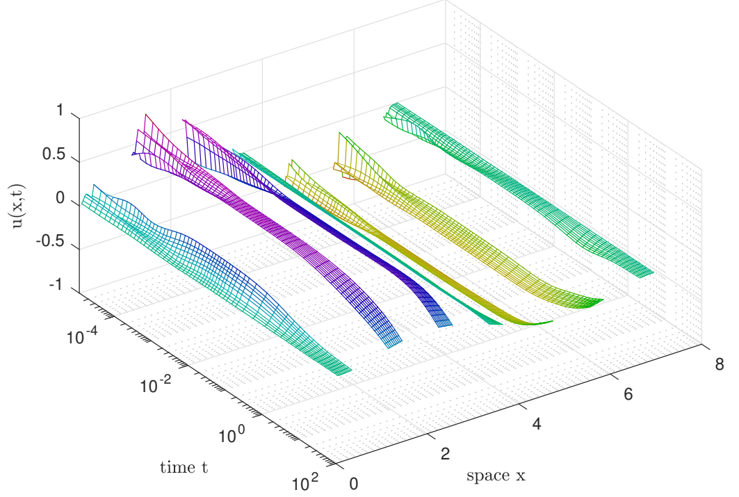
Figure 3.28: hyper-diffusing field u(x,t) in the patch scheme applied to microscale heterogeneous hyper-diffusion (Section 3.12). The log-time axis shows: t < 10^{-2} , rapid decay of sub-patch micro-structure; 10^{-2} < t < 1 , meso-time quasi-equilibrium; and 1 < t < 10^2 , slow decay of macroscale structures.
