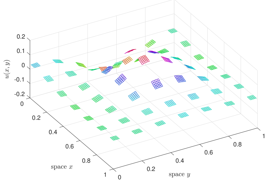
Figure 4.10: Equilibrium of the macroscale diffusion problem of Bonizzoni et al. with Neumann boundary conditions of zero (Section 4.8). Here the patches have a equispaced spatial distribution. The microscale periodicity, and hence the patch size, is chosen large enough to see within.
