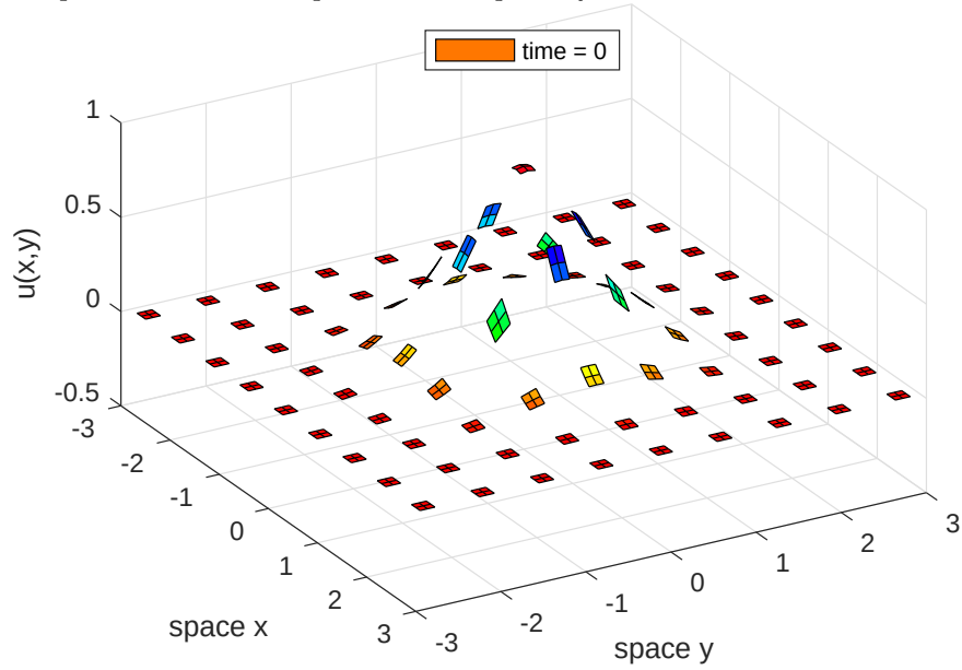
Figure 4.3: initial field u(x,y,t) at time t = 0 of the patch scheme applied to the simple wave PDE: ?? plots the computed field at time t = 2 .
