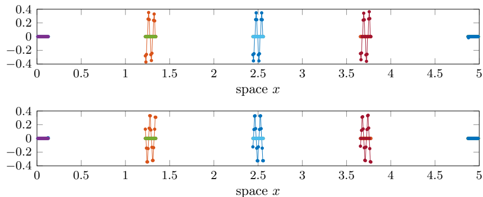
Figure 3.34: sparse basis approximations for the invariant subspace of the six slow modes of Figure 3.24. A replot of Figure 3.25 but with three of the basis vectors superimposed in each of the two panels.
