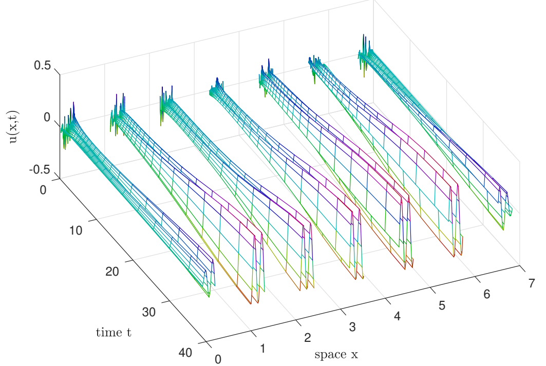
Figure 3.29: the pattern forming field u(x, t) in the patch (gap-tooth) scheme applied to a microscale discretisation of the Swift–Hohenberg PDE (Section 3.13). Physically we see the rapid decay of much microstructure, but also the meso-time growth of sub-patch-scale patterns, wavenumber k_0 , that are modulated over the inter-patch distances and over long times.
