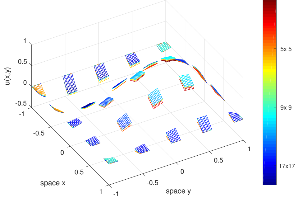
Figure 4.7: For various numbers of patches as indicated on the colorbar, plot the equilibrium of the multiscale diffusion problem of Freese with Dirichlet zero-value boundary conditions (Section 4.6). We only compare solutions only in these 25 common patches.
