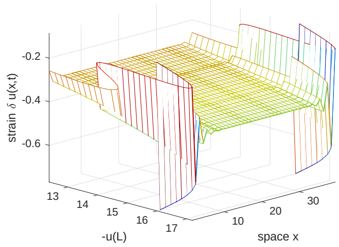
Figure 3.24: the case of microscale ‘instability’ appears as fluctuations close to both boundaries. As the system is physically compressed, the equilibrium curve has complicated folds, as shown here (and Figure 3.19(b)).
