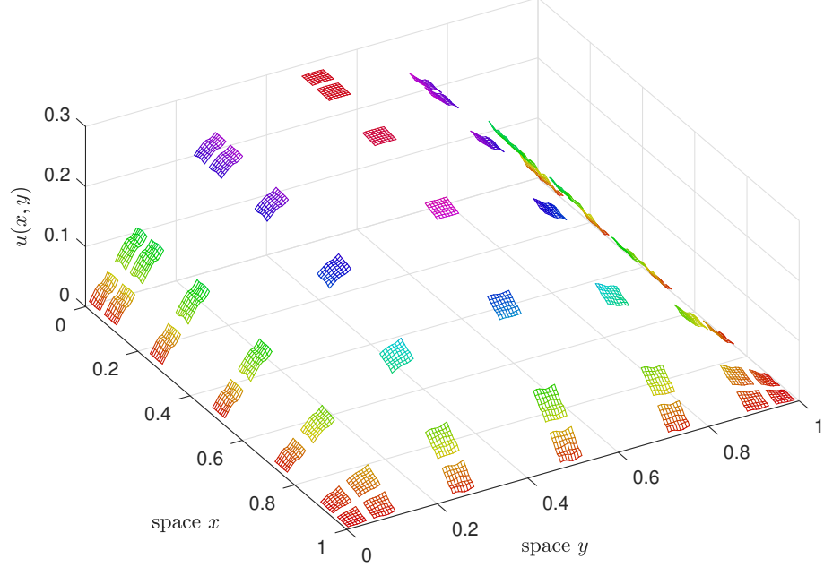
Figure 4.9: Equilibrium of the macroscale diffusion problem of Abdulle with boundary conditions of Dirichlet zero-value except for x = 0 which is Neumann (Section 4.7). Here the patches have a Chebyshev-like spatial distribution. The patch size is chosen large enough to see within.
