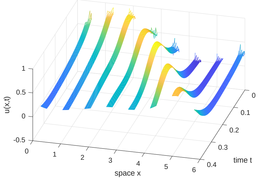
Figure 3.8: a short time simulation of the Burgers' map (??) on patches in space. It requires many very small time-steps only just visible in this mesh.
