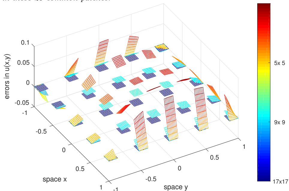
Figure 4.8: For various numbers of patches as indicated on the colorbar, plot the equilibrium of the multiscale diffusion problem of Freese with Dirichlet zero-value boundary conditions (Section 4.6). We only compare solutions only in these 25 common patches.
