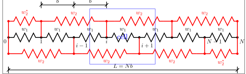
Figure 3.15: 1D arrangement of non-linear springs with connections to (a) next-to-neighbour node (Combescure 2022, Fig. 3(a)). The blue box is one micro-cell of one period, width 2b , containing an odd and an even i .
