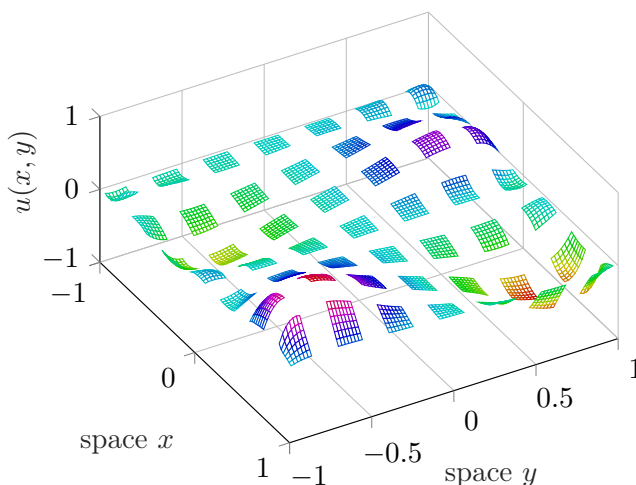
Figure 4.4: Equilibrium of the multiscale diffusion problem of Freese with Dirichlet zero-value boundary conditions (Section 4.5). The patch size is not small so we can see the patches and the sub-patch grid. The solution u(x, y) is boringly smooth.
