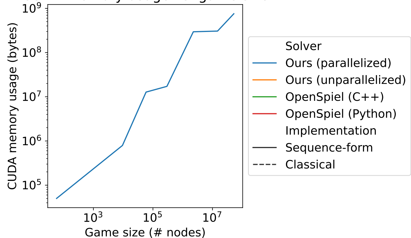
CUDA memory usage vs. game size
