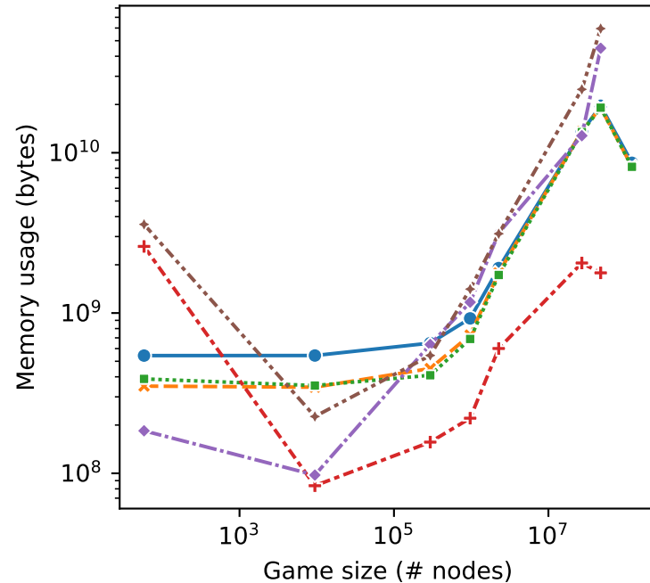
Memory usage
