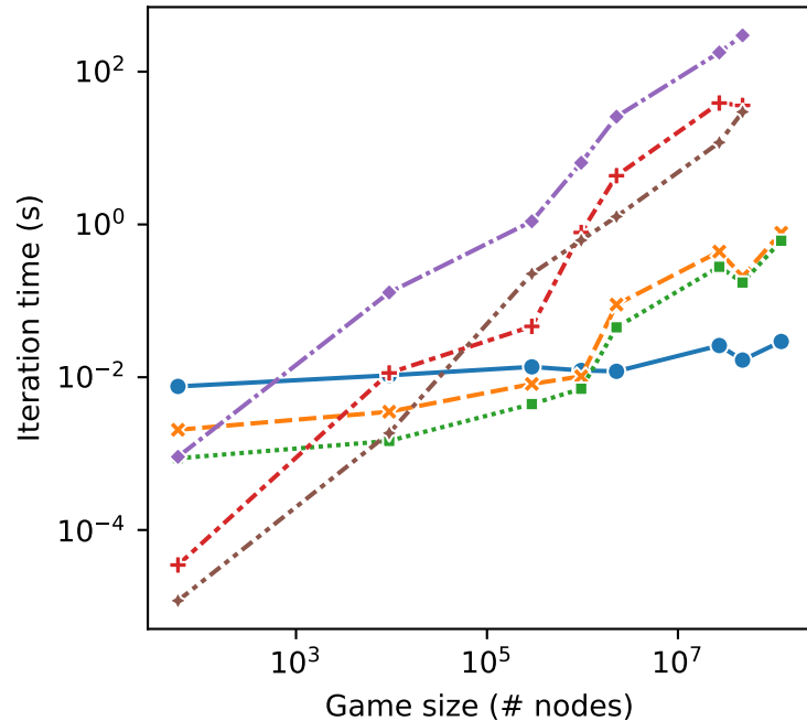
Iteration time
