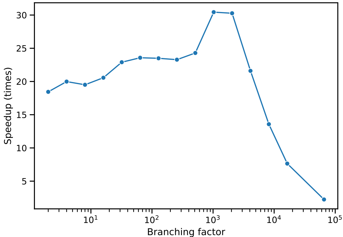
Speedup vs. branching factor
