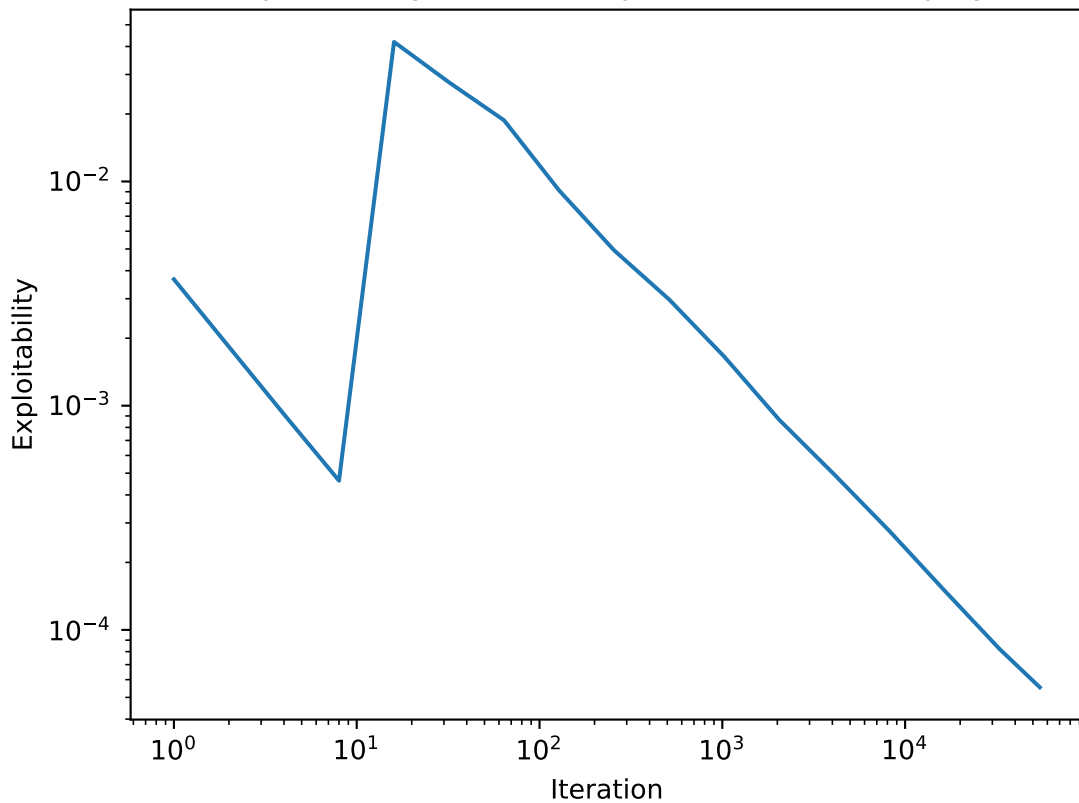
Exploitability of battleship (medium) in self-play
