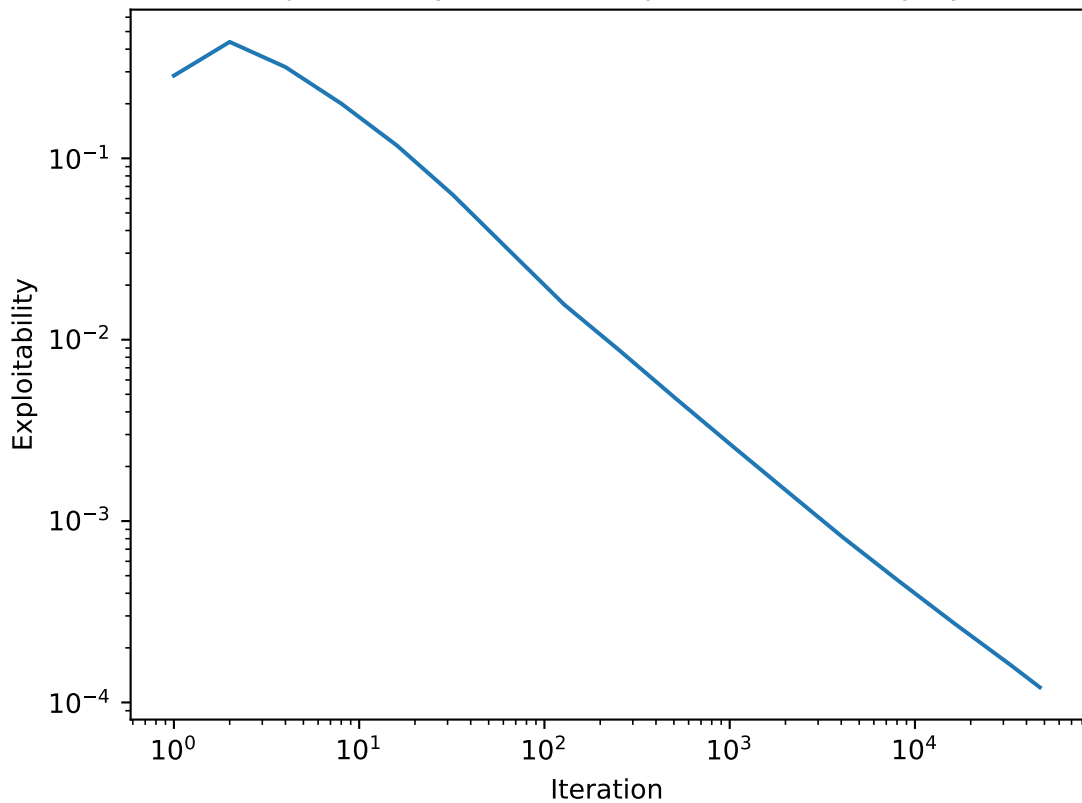
Exploitability of battleship (small) in self-play
