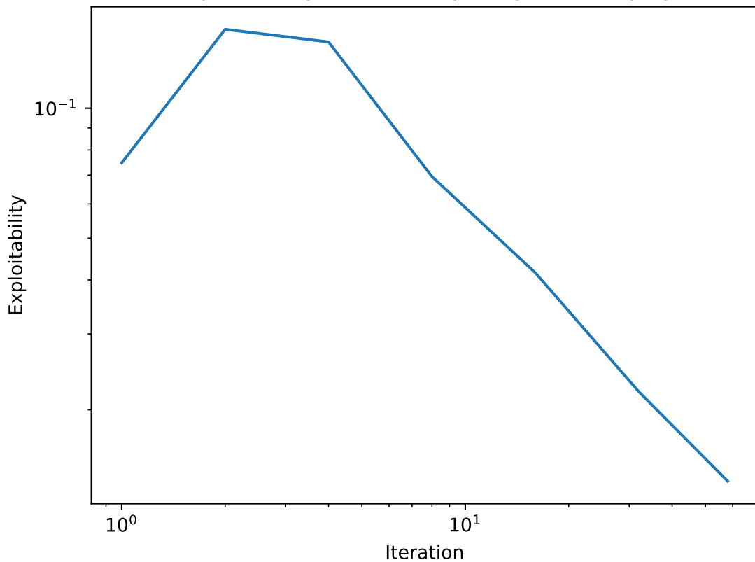
Exploitability of battleship (large) in self-play
