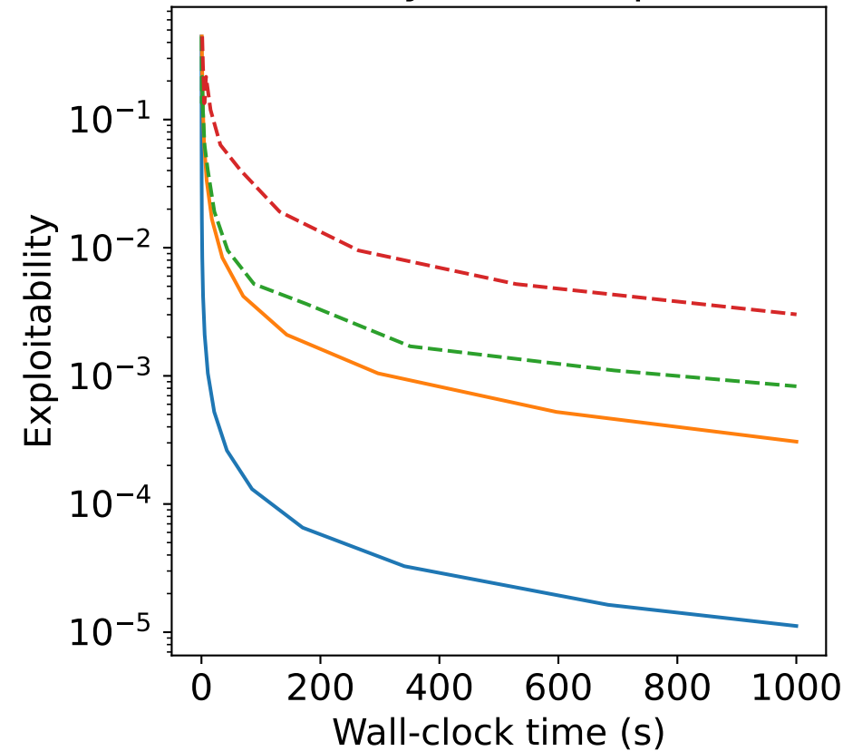
Tiny battleship
