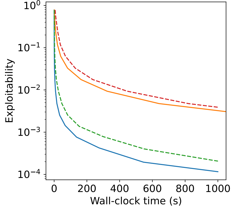
Liar's dice
