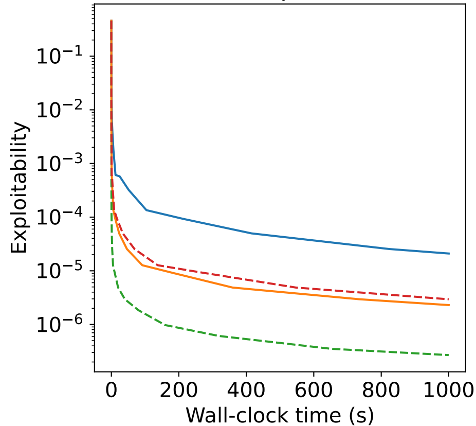
Kuhn poker
