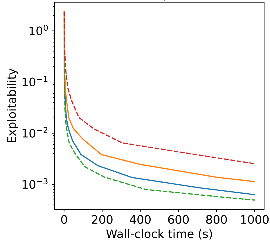
Leduc poker
