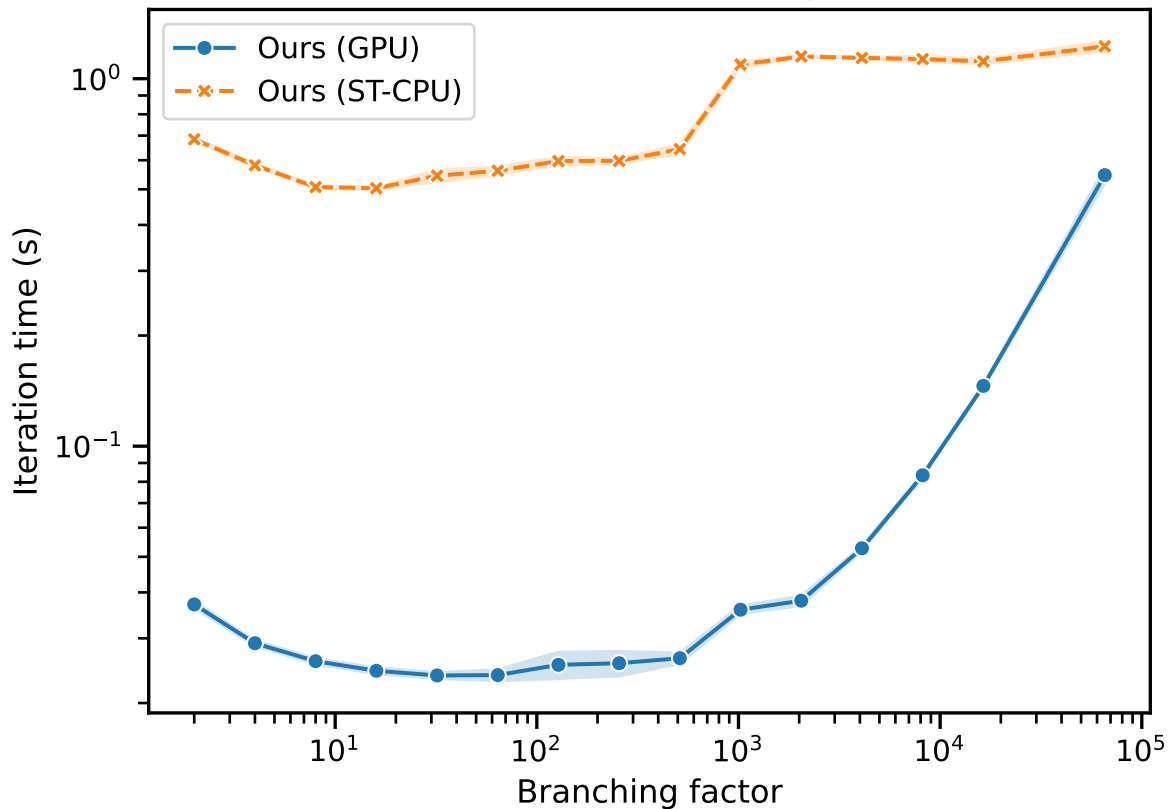
Iteration time vs. branching factor
