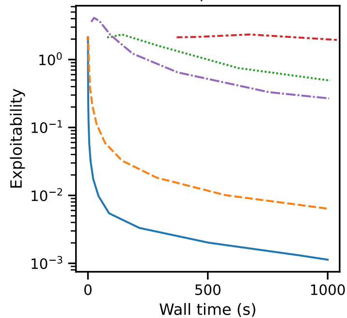
Battleship-3x2-22-3
