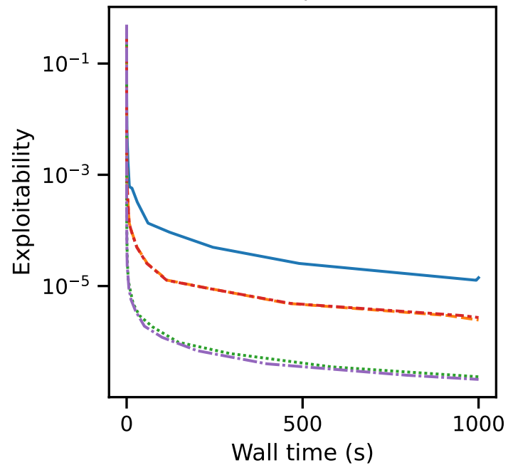
Kuhn poker
