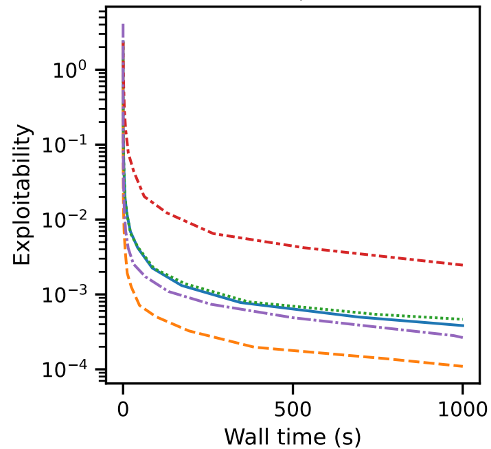
Leduc poker
