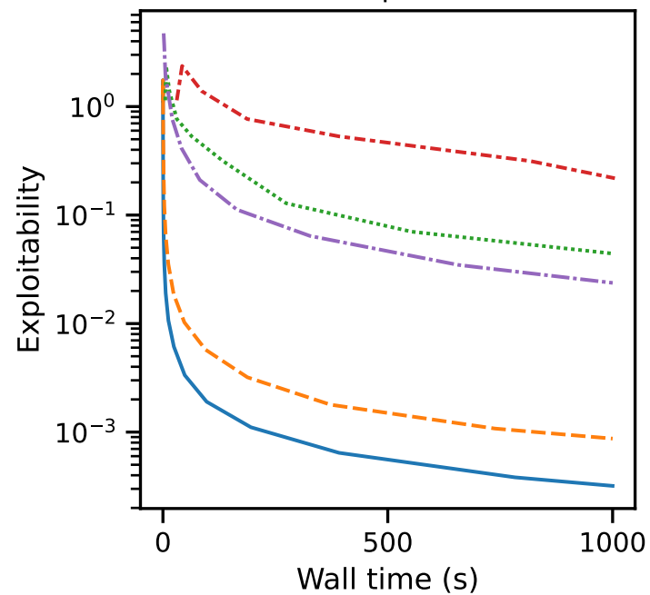
Battleship-3x2-2-3
