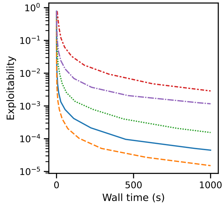
Liar's dice
