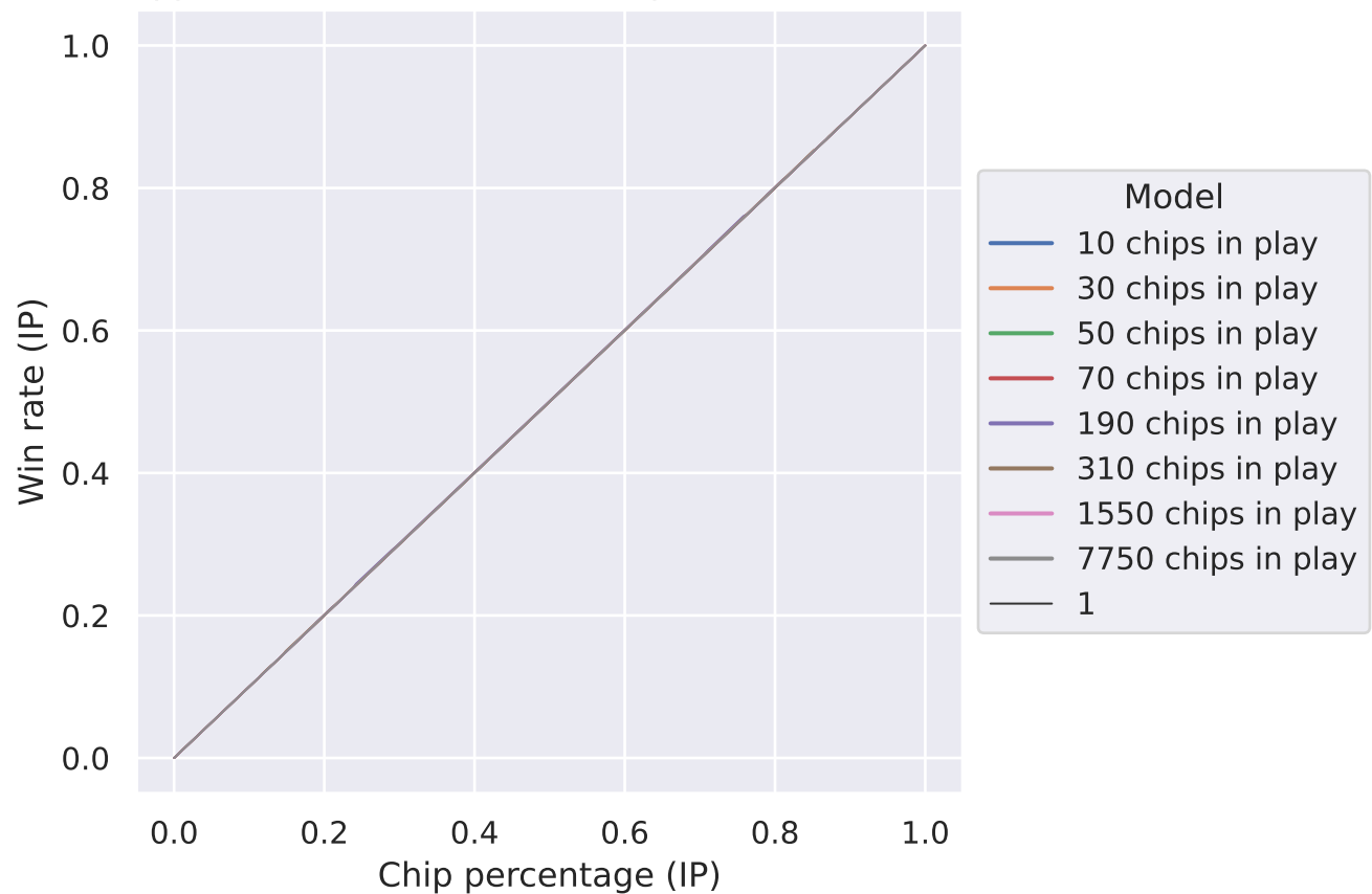
Approximated win rates (IP) of poker tournaments
