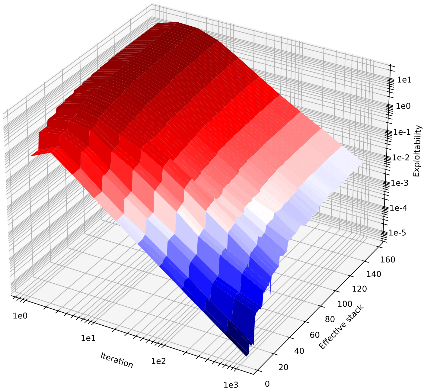
Exploitabilities of CFR+ in self-play
