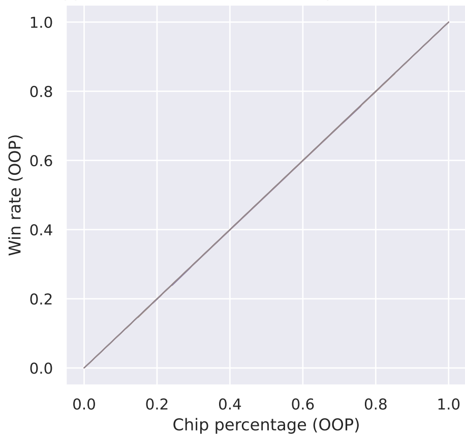
Approximated win rates (OOP) of poker tournaments
