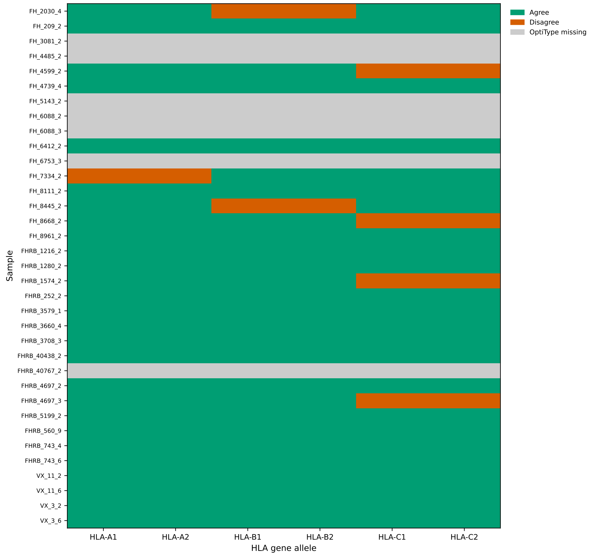
scRNA HLA typing: OptiType vs arcasHLA concordance (FIMM cohort)
