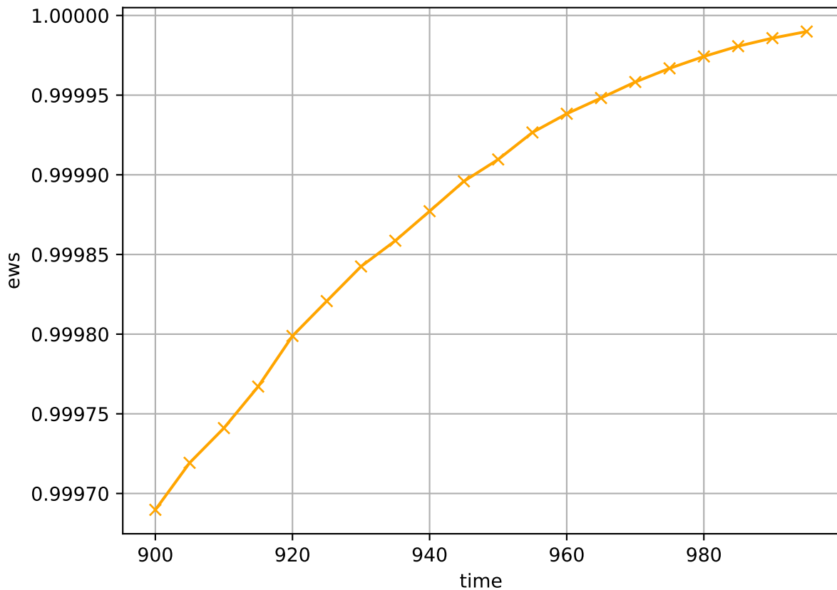
kendall tau 1.0
