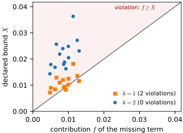
(a) sealed replica, 14 sub-support claims (diagnostic)
