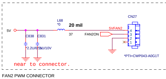
FAN2 PWM CONNECTOR
