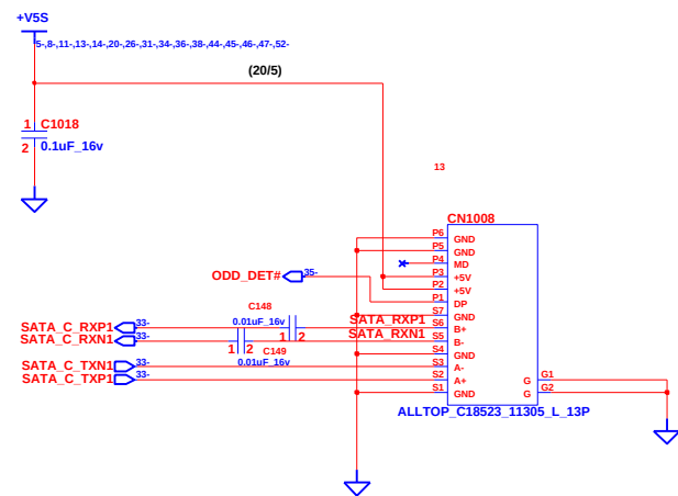
SATA ODD
