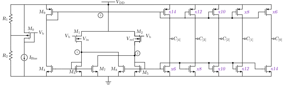
Figure 3.9: Bulk-driven OTA of the third architecture [10], with the function of each transistor annotated, the non-tailed bulk-driven input pair M_1 , M_2 , the current-mirror loads and the cross-coupled load M_7 , M_8 that provides the local positive feedback. The circled points 1 and 2 mark the two differential output nodes and point 3 the supply-side node of the input pair.
