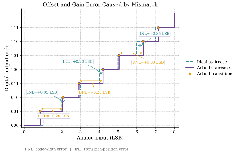
Figure 2.1: Effect of device mismatch on the ADC transfer characteristic. The actual staircase departs from the ideal one, the deviation in each code width is the differential non-linearity (DNL) and the displacement of each transition from its ideal position is the integral non-linearity (INL).
