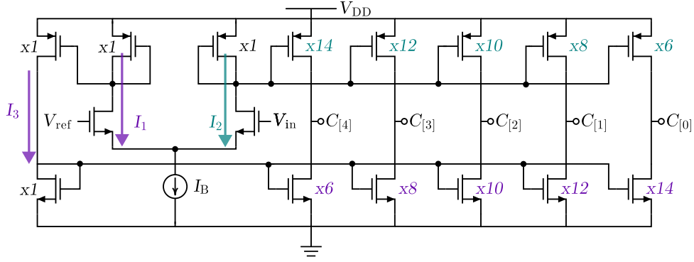
Figure 3.2: Transistor-level schematic of the first architecture, the current-mirror Flash ADC, showing the differential input pair driven by V_{\text{ref}} and V_{\text{in}} , the tail current source I_B and the five current-mirror output branches whose PMOS and NMOS width ratios set the thermometer thresholds C[4] down to C[0] .
