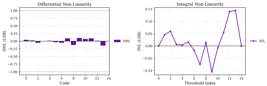
Figure 3.14: DNL per code (left) and INL per transition (right) of the final architecture at the typical (TT) corner.
