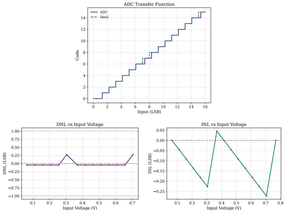
Figure 4.7: Static characterisation of the synchronous reference: (top) measured transfer function against the ideal staircase, (bottom left) DNL per code and (bottom right) INL per transition.
